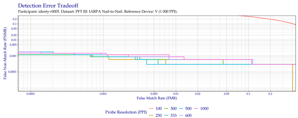
Figure 17: Detection error tradeoff of comparisons from the PFT III IARPA N2N dataset using downsampled probe images of various resolutions as compared to 1 000 (native) images.
