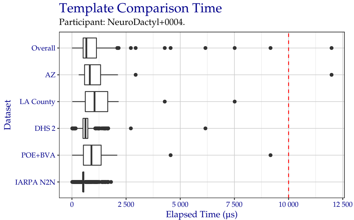
Figure 3: Box plots of elapsed microseconds when comparing two templates from a fixed sample of data from the PFT III evaluation. All times are used, even if a failure occurred. Tabular versions of this data are shown in Table 5.
