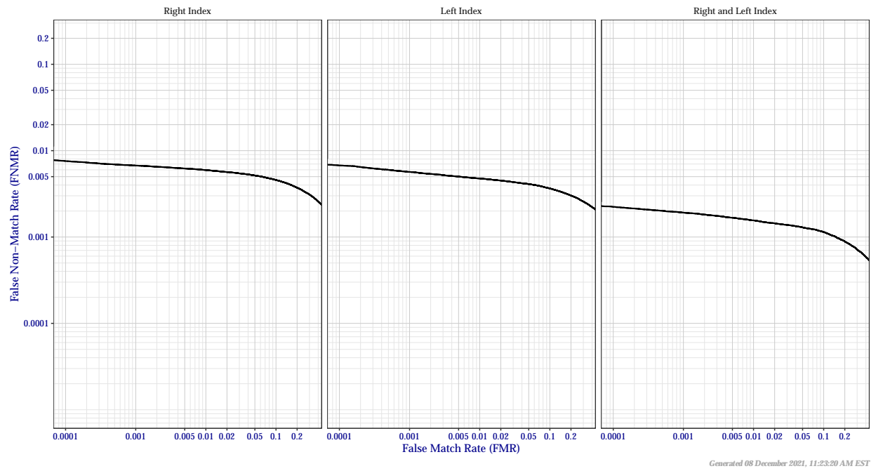
Figure 13: Detection error tradeoff of comparisons from the PFT III VISIT2 dataset, separated by finger position. Combined finger positions were generated by sum fusion.
