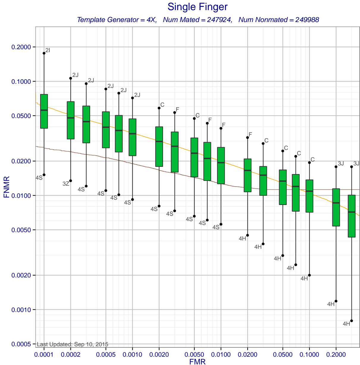
Figure 2: Single finger DET statistics for template generator 4X. Each box shows the distribution of FNMRs at a fixed FMR across different matchers. The whisker ends show the minimum and maximum FNMRs. The brown curve shows the DET curve when the matcher and template generators were submitted by the same participant. The orange DET curve shows pooled performance when all matchers compare templates created by 4X.
