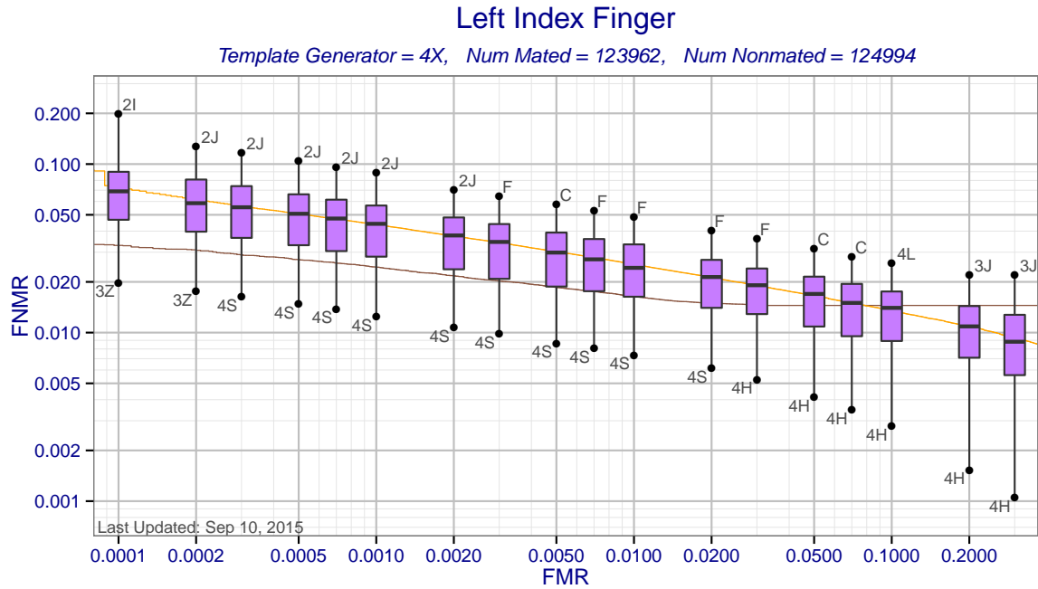
Figure 4: Left Index Finger DET statistics for template generator 4X. Each box shows the distribution of FNMRs at a fixed FMR across different template generators. The brown curve shows the DET curve when the matcher and template generators were submitted by the same participant. The orange DET curve shows pooled performance when all matchers use templates created by 4X.
