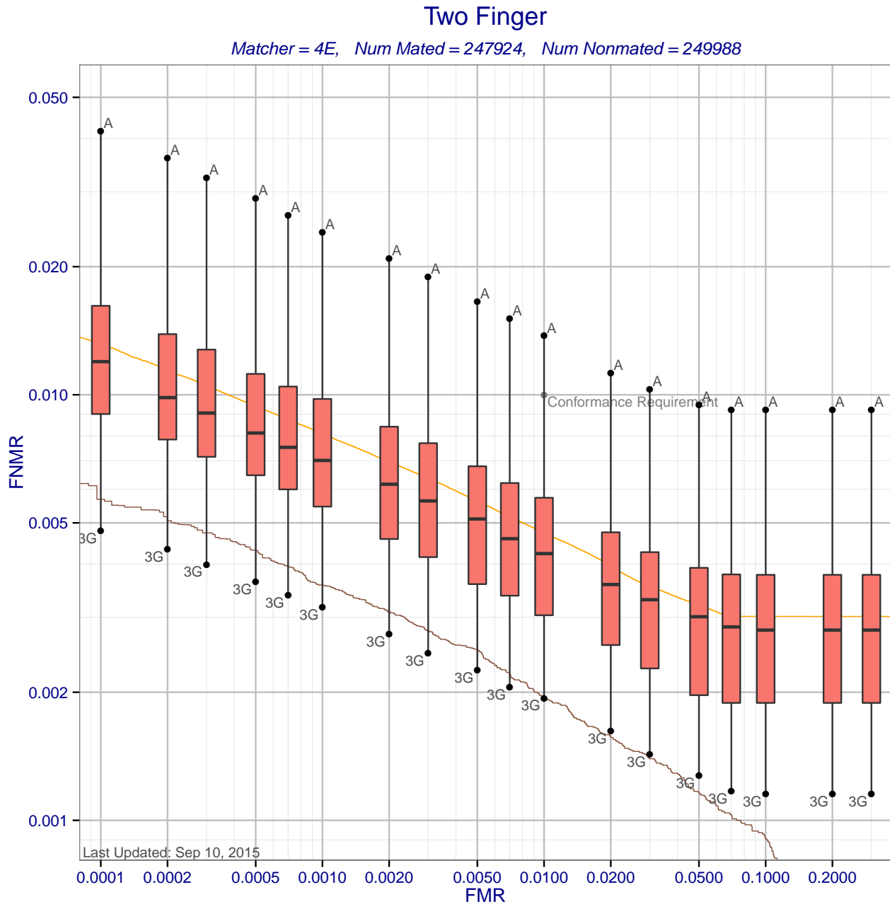
Figure 7: Two finger DET statistics for matcher 4E. Each box shows the distribution of FNMRs at a fixed FMR across all MINEX compliant template generators. The whisker ends show the minimum and maximum FNMRs. The orange DET curve shows pooled performance against all template generators. Score-level fusion is achieved by averaging the scores for left and right index fingers.
