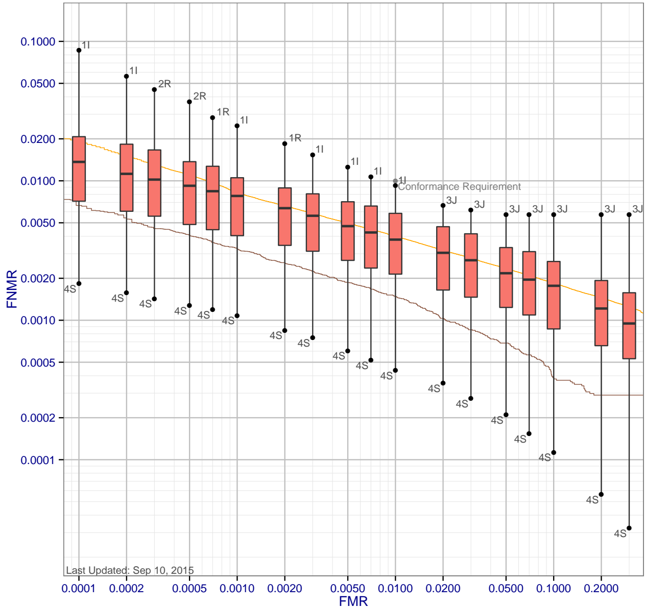
Figure 6: Two Finger DET statistics for template generator 2I. Each box shows the distribution of FNMRs at a fixed FMR across different matchers. The whisker ends show the minimum and maximum FNMRs. The brown curve shows the DET curve when the matcher and template generators were submitted by the same participant. The orange DET curve shows pooled performance when all matchers use templates created by 2I. Score-level fusion is achieved by averaging the scores for left and right index fingers.
