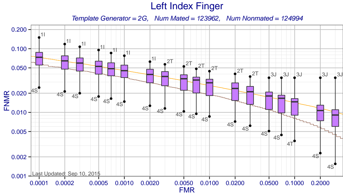
Figure 4: Left Index Finger DET statistics for template generator 2G. Each box shows the distribution of FNMRs at a fixed FMR across different template generators. The brown curve shows the DET curve when the matcher and template generators were submitted by the same participant. The orange DET curve shows pooled performance when all matchers use templates created by 2G.
