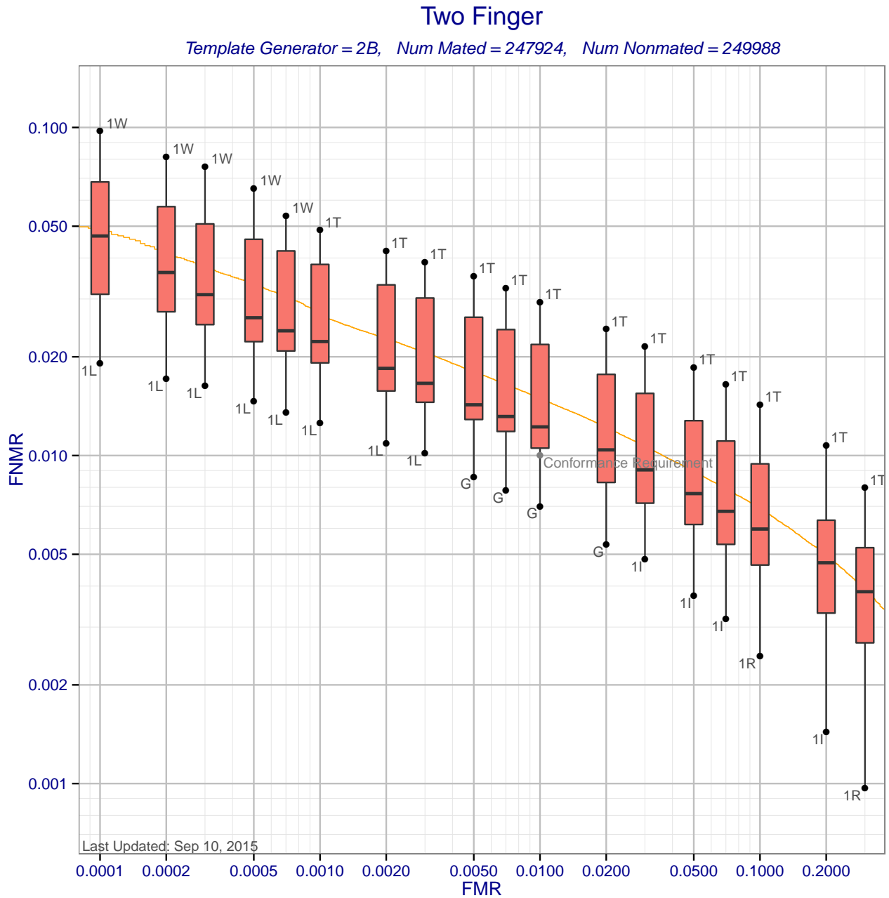
Figure 6: Two Finger DET statistics for template generator 2B. Each box shows the distribution of FNMRs at a fixed FMR across different matchers. The whisker ends show the minimum and maximum FNMRs. The orange DET curve shows pooled performance when all matchers use templates created by 2B. Score-level fusion is achieved by averaging the scores for left and right index fingers.
