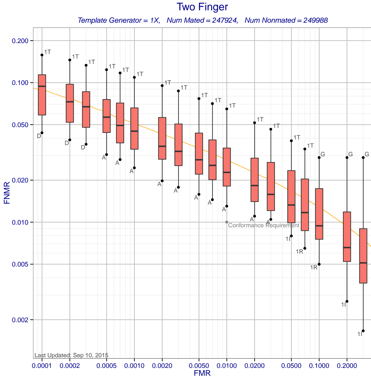
Figure 6: Two Finger DET statistics for template generator 1X. Each box shows the distribution of FNMRs at a fixed FMR across different matchers. The whisker ends show the minimum and maximum FNMRs. The brown curve shows the DET curve when the matcher and template generators were submitted by the same participant. The orange DET curve shows pooled performance when all matchers use templates created by 1X. Score-level fusion is achieved by averaging the scores for left and right index fingers.
