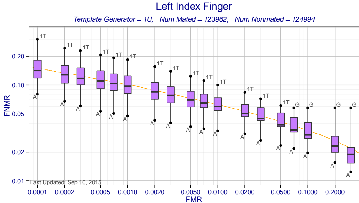
Figure 4: Left Index Finger DET statistics for template generator 1U. Each box shows the distribution of FNMNRs at a fixed FMR across different template generators. The brown curve shows the DET curve when the matcher and template generators were submitted by the same participant. The orange DET curve shows pooled performance when all matchers use templates created by 1U.
