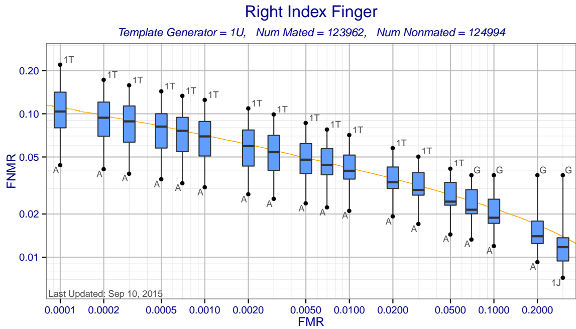
Figure 3: Right Index Finger DET statistics for template generator 1U. Each box shows the distribution of FNMNRs at a fixed FMR across different matchers. The whisker ends show the minimum and maximum FNMNRs. The brown curve shows the DET curve when the matcher and template generators were submitted by the same participant. The orange DET curve shows pooled performance when all matchers use templates created by 1U.
