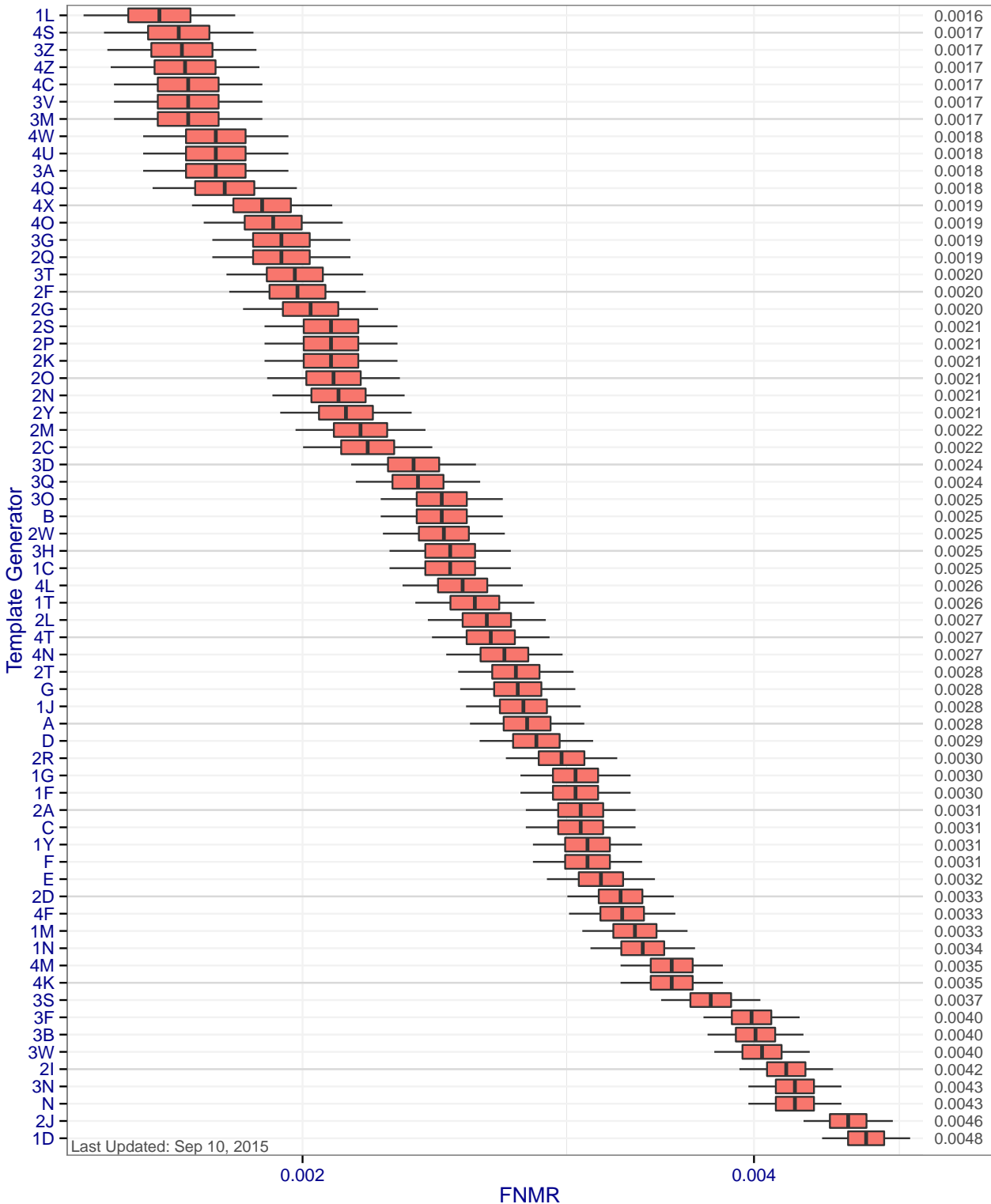
Figure 8: Two finger FNMR at FMR=0.01 when matcher 1L compares templates created by different template generators. Each box represents uncertainty about the true FNMR. The box edges mark the 50% confidence intervals while the whiskers mark the 90% confidence intervals. The numbers on the right show the actual computed FNMRs. Score-level fusion is achieved by averaging the scores for left and right index fingers.
