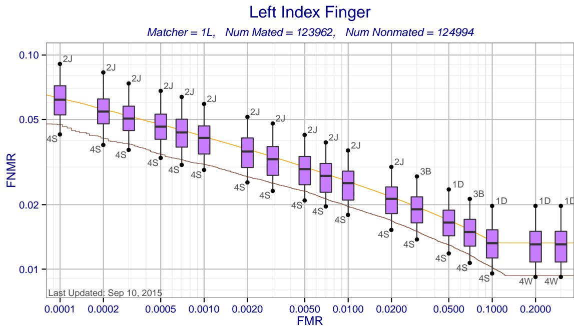
Figure 4: Left index finger DET statistics for matcher 1L. Each box shows the distribution of FNMNRs at a fixed FMR across all MINEX compliant template generators. The ends of whiskers show the minimum and maximum FNMNRs. The orange DET curve shows pooled performance against all template generators.
