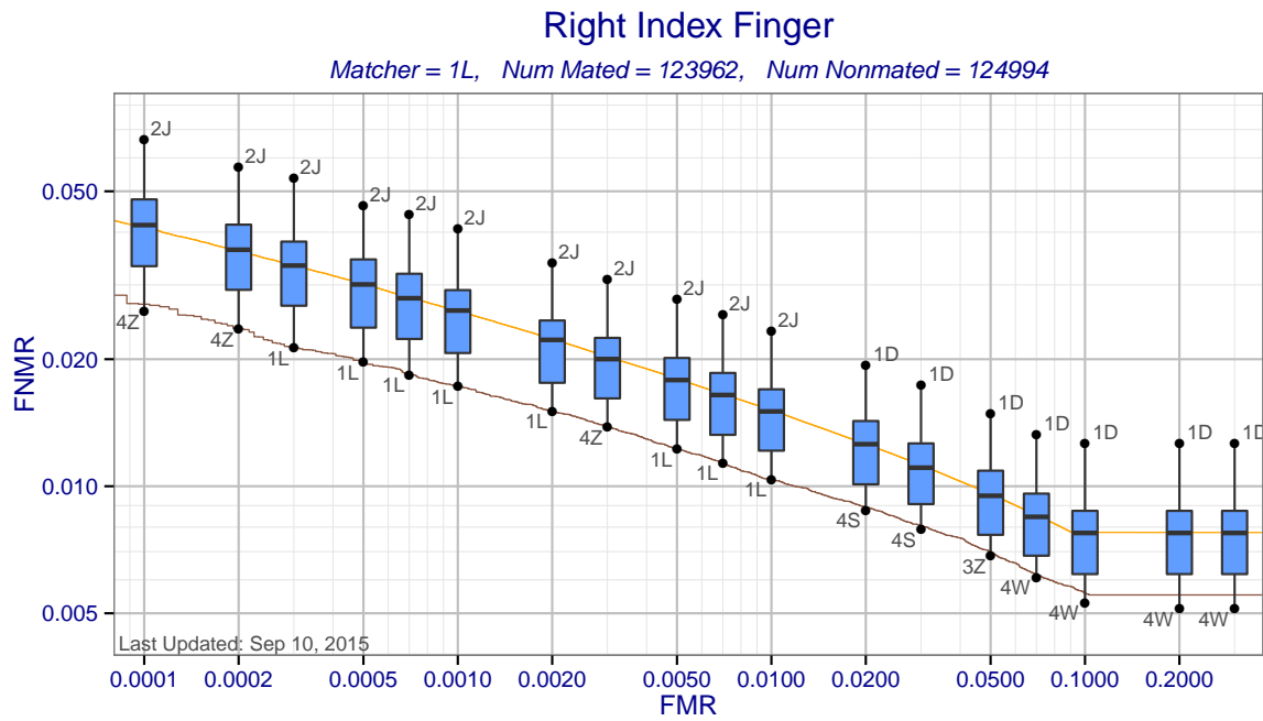
Figure 3: Right index finger DET statistics for matcher 1L. Each box shows the distribution of FNMNR at a fixed FMR across all MINEX compliant template generators. The ends of the whiskers show the minimum and maximum FNMNRs. The orange DET curve shows pooled performance against all template generators.
