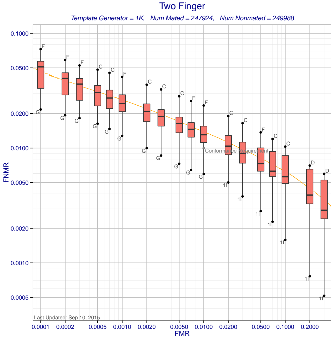
Figure 6: Two Finger DET statistics for template generator 1K. Each box shows the distribution of FNMRs at a fixed FMR across different matchers. The whisker ends show the minimum and maximum FNMRs. The brown curve shows the DET curve when the matcher and template generators were submitted by the same participant. The orange DET curve shows pooled performance when all matchers use templates created by 1K. Score-level fusion is achieved by averaging the scores for left and right index fingers.
