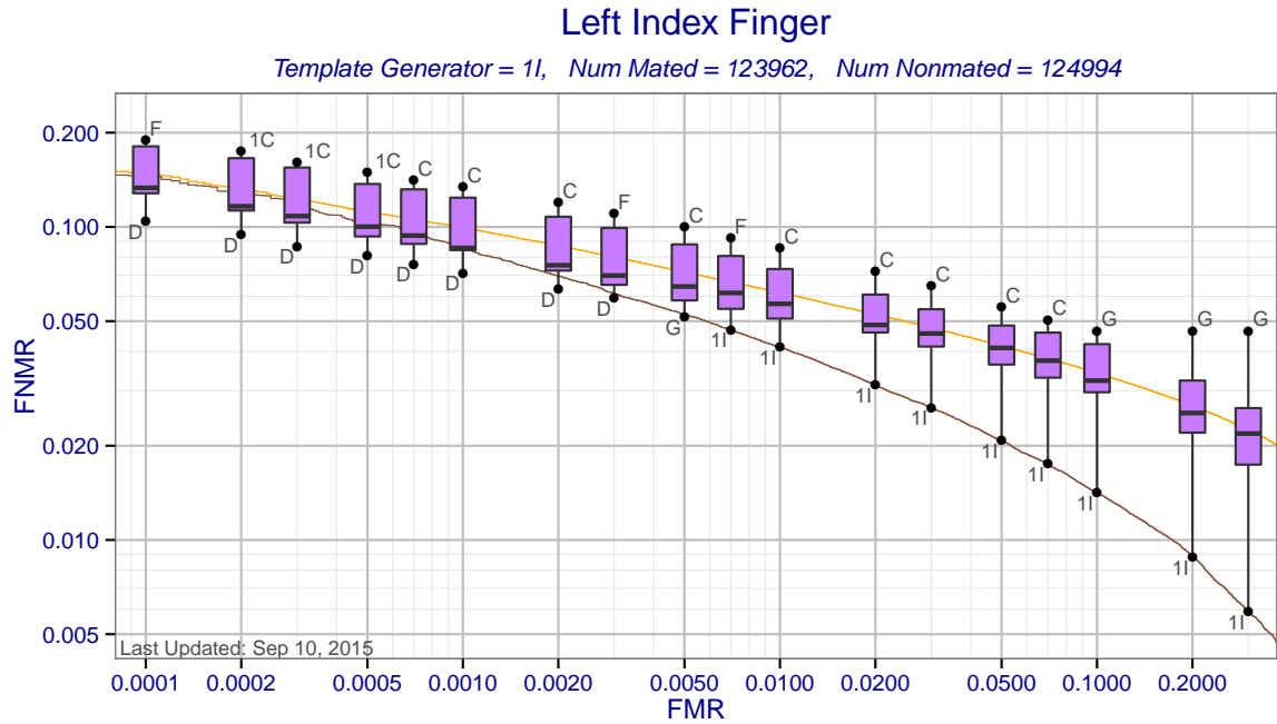
Figure 4: Left Index Finger DET statistics for template generator 1I. Each box shows the distribution of FNMRs at a fixed FMR across different template generators. The brown curve shows the DET curve when the matcher and template generators were submitted by the same participant. The orange DET curve shows pooled performance when all matchers use templates created by 1I.
