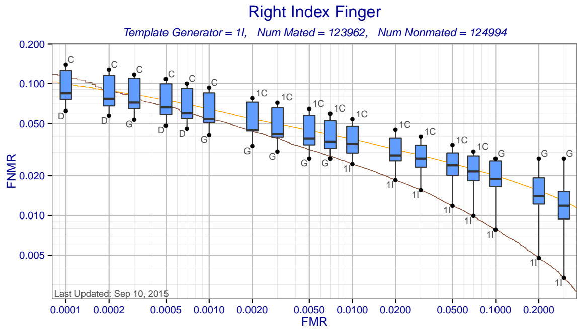
Figure 3: Right Index Finger DET statistics for template generator 1I. Each box shows the distribution of FNMRs at a fixed FMR across different matchers. The whisker ends show the minimum and maximum FNMRs. The brown curve shows the DET curve when the matcher and template generators were submitted by the same participant. The orange DET curve shows pooled performance when all matchers use templates created by 1I.
