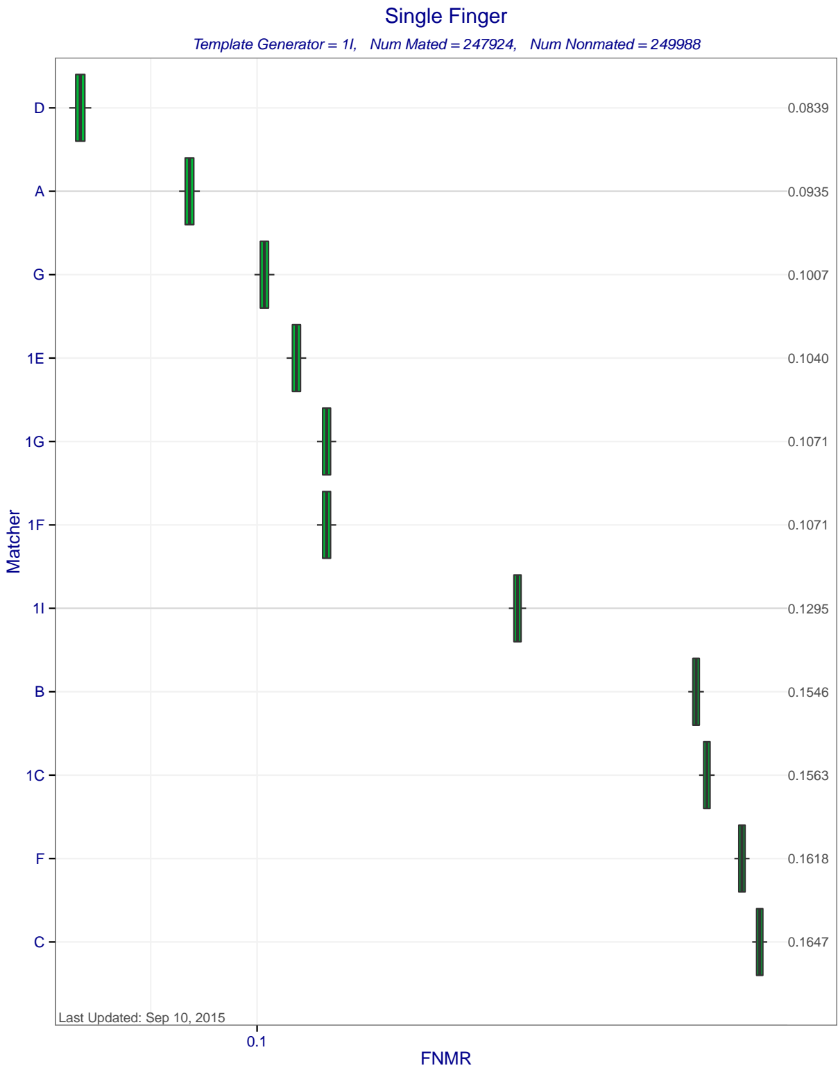
Figure 5: Single Finger FNMRs at FMR=0.0001 when MINEX compliant matchers compare templates created by template generator 1I. Each box represents uncertainty about the true FNMR. The box edges mark the 50% confidence intervals while the whiskers mark the 90% confidence intervals. The numbers on the right show the actual computed FNMRs.
