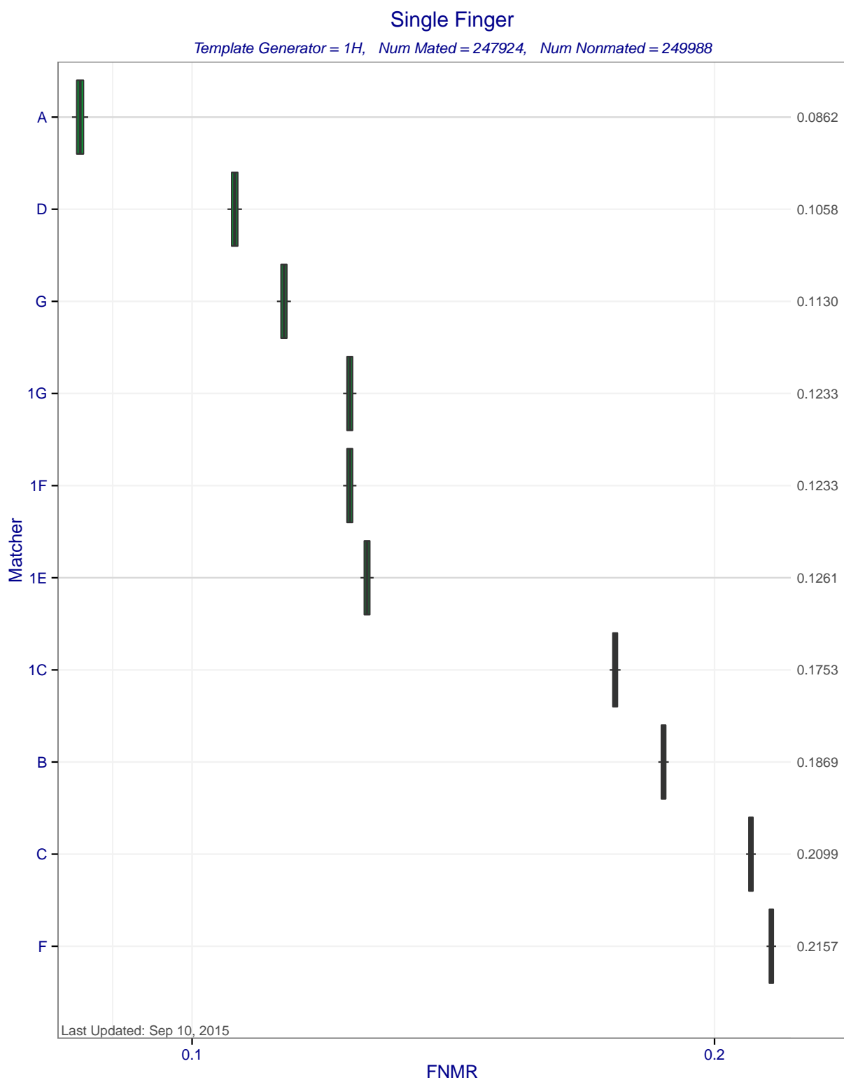
Figure 5: Single Finger FNMRs at FMR=0.0001 when MINEX compliant matchers compare templates created by template generator 1H. Each box represents uncertainty about the true FNMR. The box edges mark the 50% confidence intervals while the whiskers mark the 90% confidence intervals. The numbers on the right show the actual computed FNMRs.
