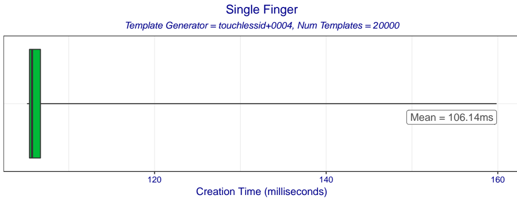
Figure 2: Boxplot of template creation times for template generator touchlessid+0004. The box edges mark the 10th and 90th percentiles while the whiskers mark the maximum and minimum creation times.
