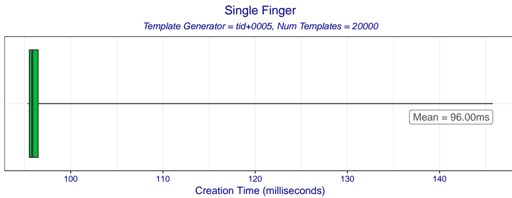
Figure 2: Boxplot of template creation times for template generator tid+0005. The box edges mark the 10th and 90th percentiles while the whiskers mark the maximum and minimum creation times.
