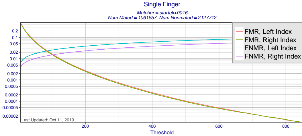
Figure 11: Single finger FMR and FNMR as a function of score threshold for matcher startek+0016 using templates created by all MINEX III compliant template generators. Separate curves are presented for left and right index fingers.
