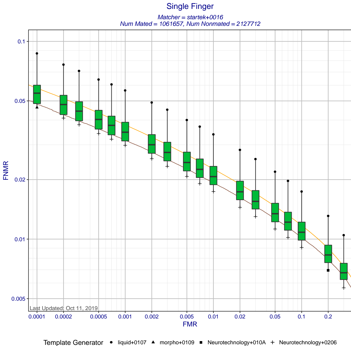
Figure 2: Single finger DET statistics for matcher startek+0016. Each box shows the distribution of FNMRs at a fixed FMR across all MINEX III compliant template generators. The ends of the whiskers show the minimum and maximum FNMRs. The orange DET curve shows pooled performance against all template generators.
