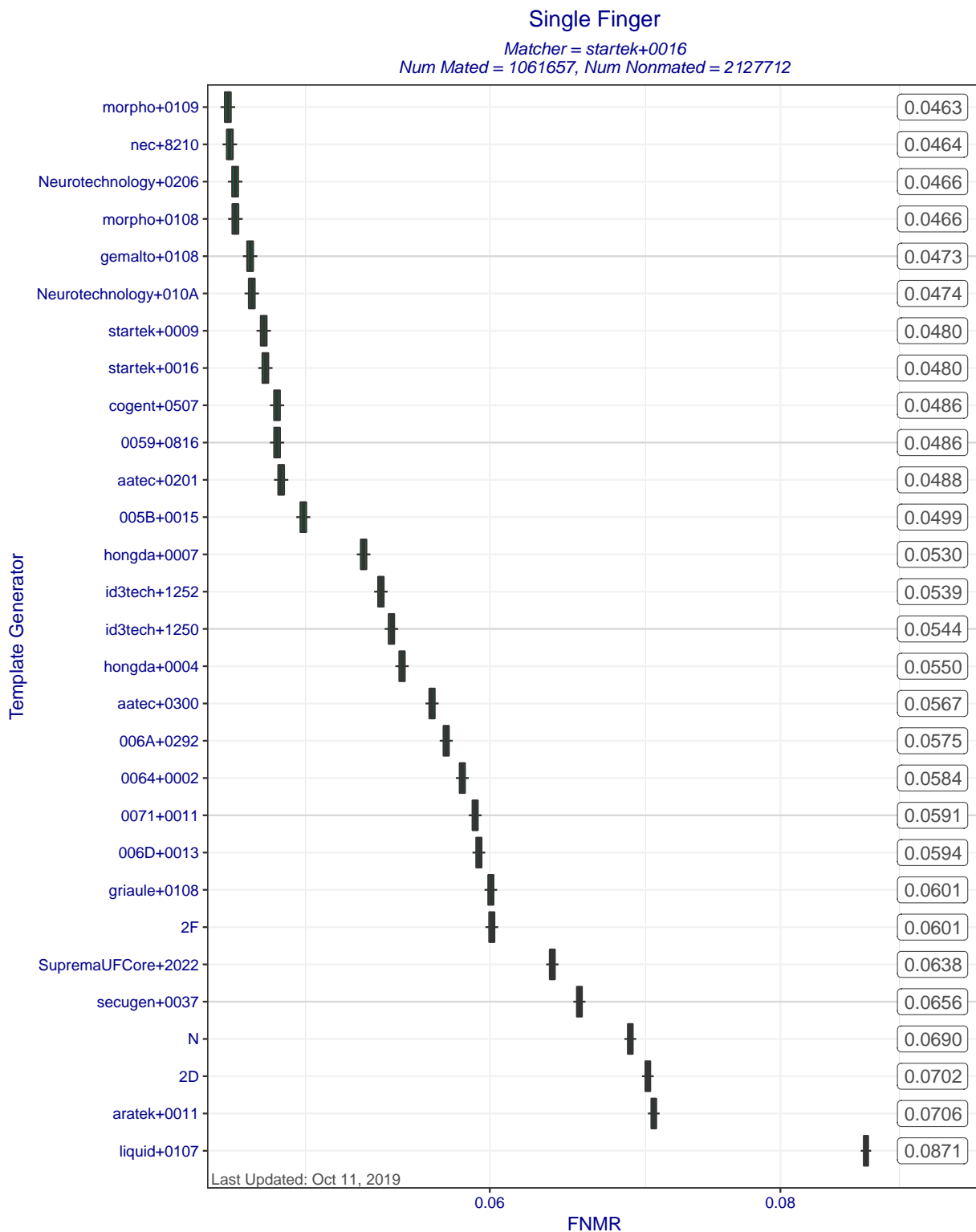
Figure 5: Single finger FNMRs at FMR = 0.0001 when matcher startek+0016 compares templates created by different template generators. The ends of the whiskers show the minimum and maximum FNMRs. Each box represents uncertainty about the true FNMR. The box edges mark the 50% confidence intervals while the whiskers mark the 90% confidence intervals. The numbers on the right show the actual computed FNMRs.
