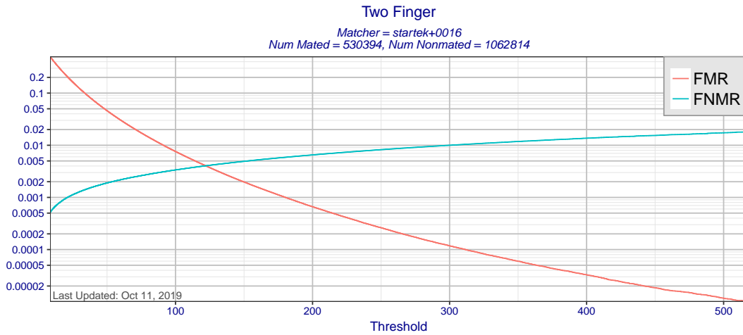
Figure 12: Two finger FMR and FNMR as a function of score threshold for matcher startek+0016 using templates created by all MINEX III compliant template generators. Score-level fusion is achieved by averaging scores for the left and right index fingers.
