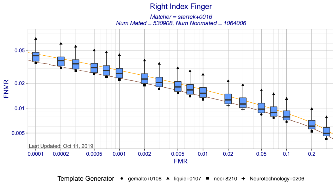
Figure 3: Right index finger DET statistics for matcher startek+0016. Each box shows the distribution of FNMR at a fixed FMR across all MINEX III compliant template generators. The ends of the whiskers show the minimum and maximum FNMRs. The orange DET curve shows pooled performance against all template generators.
