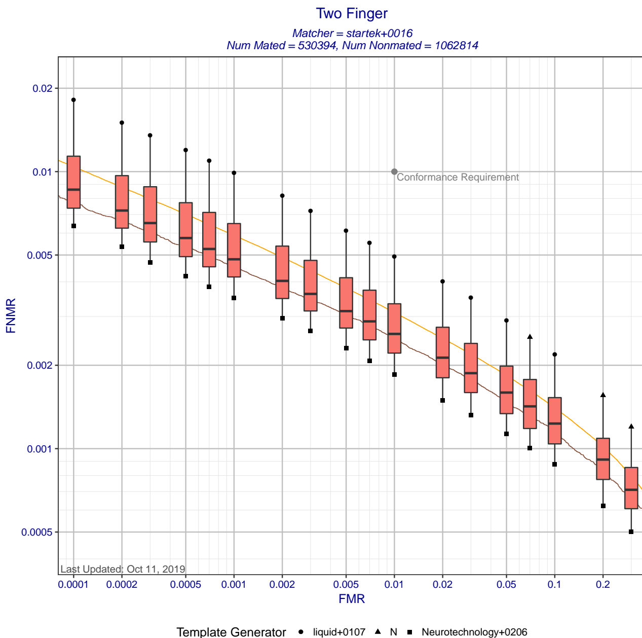
Figure 7: Two finger DET statistics for matcher startek+0016. Each box shows the distribution of FNMRs at a fixed FMR across all MINEX III compliant template generators. The whisker ends show the minimum and maximum FNMRs. The orange DET curve shows pooled performance against all template generators. Score-level fusion is achieved by averaging the scores for left and right index fingers.
