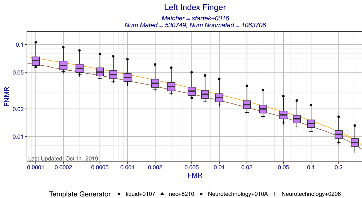
Figure 4: Left index finger DET statistics for matcher startek+0016. Each box shows the distribution of FNMRs at a fixed FMR across all MINEX III compliant template generators. The ends of whiskers show the minimum and maximum FNMRs. The orange DET curve shows pooled performance against all template generators.
