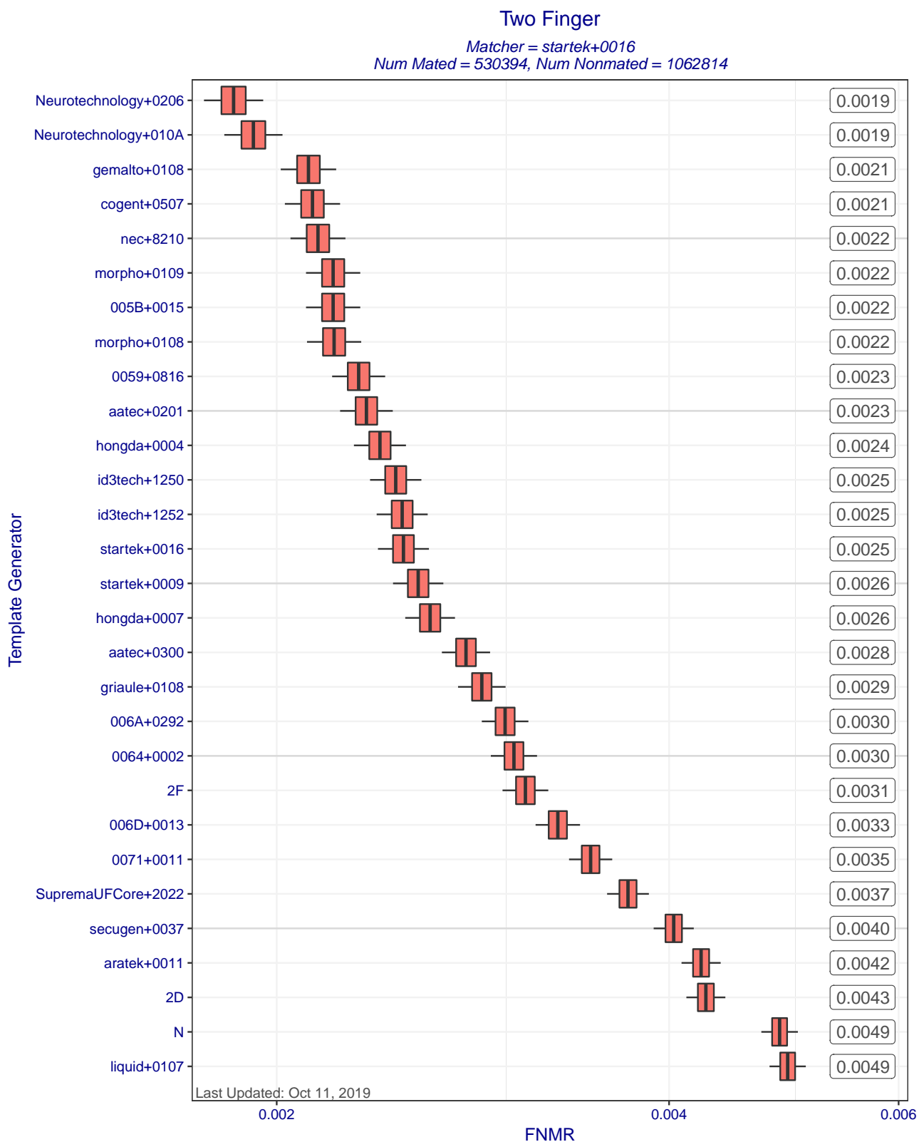
Figure 8: Two finger FNMR at FMR=0.01 when matcher startek+0016 compares templates created by different template generators. Each box represents uncertainty about the true FNMR. The box edges mark the 50% confidence intervals while the whiskers mark the 90% confidence intervals. The numbers on the right show the actual computed FNMRs. Score-level fusion is achieved by averaging the scores for left and right index fingers.
