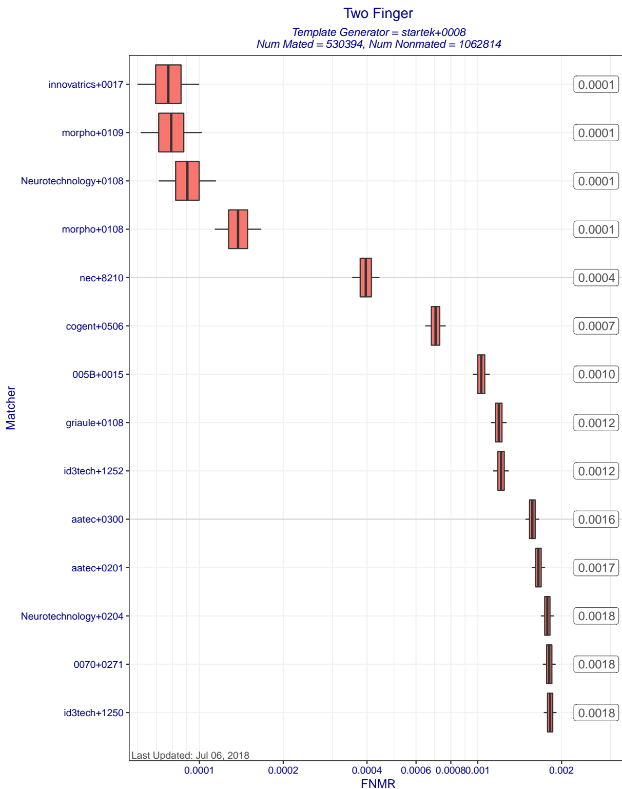
Figure 7: Two Finger FNMR at FMR=0.01 when different matchers compare templates created by template generator startek+0008. Each box represents uncertainty about the true FNMR. The box edges mark the 50% confidence intervals while the whiskers mark the 90% confidence intervals. The numbers on the right show the actual computed FNMRs. Score-level fusion is achieved by averaging the scores for left and right index fingers.
