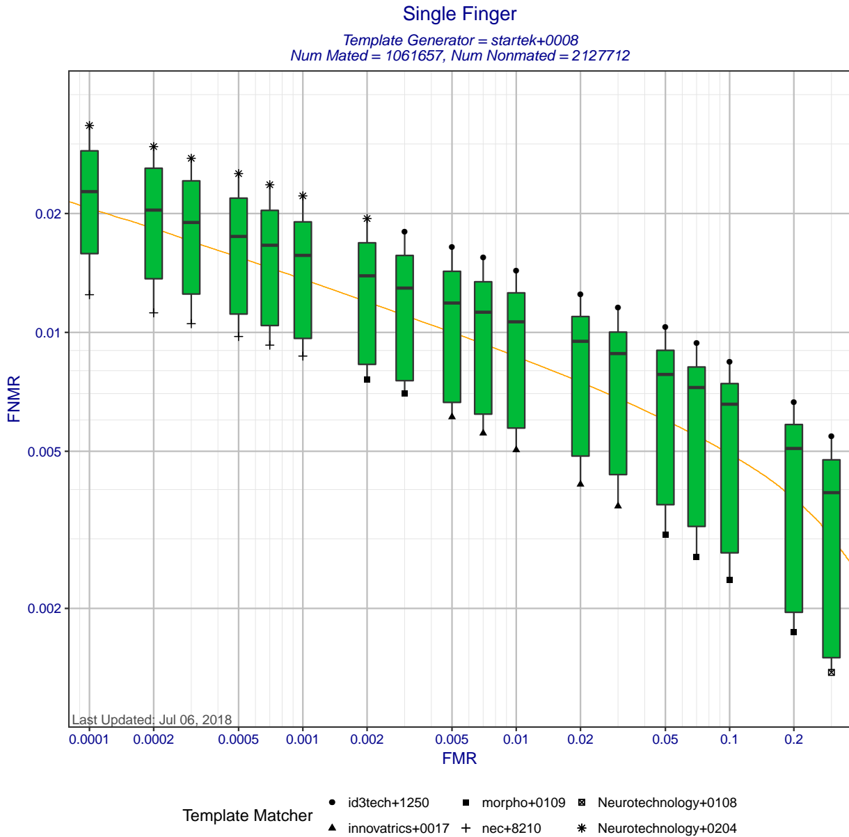
Figure 2: Single finger DET statistics for template generator startek+0008. Each box shows the distribution of FNMRs at a fixed FMR across different matchers. The whisker ends show the minimum and maximum FNMRs. The orange DET curve shows pooled performance when all matchers compare templates created by startek+0008.
