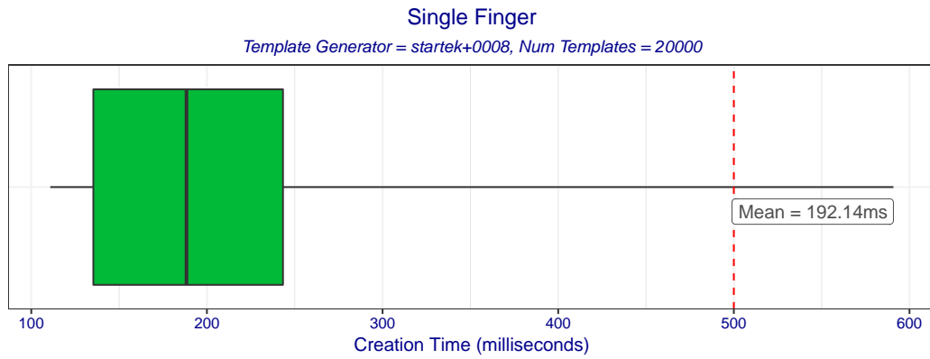
Figure 8: Boxplot of template creation times for template generator startek+0008. The box edges mark the 10th and 90th percentiles while the whiskers mark the maximum and minimum creation times.
