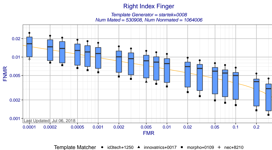
Figure 3: Right Index Finger DET statistics for template generator startek+0008. Each box shows the distribution of FNMRs at a fixed FMR across different matchers. The whisker ends show the minimum and maximum FNMRs. The orange DET curve shows pooled performance when all matchers use templates created by startek+0008.
