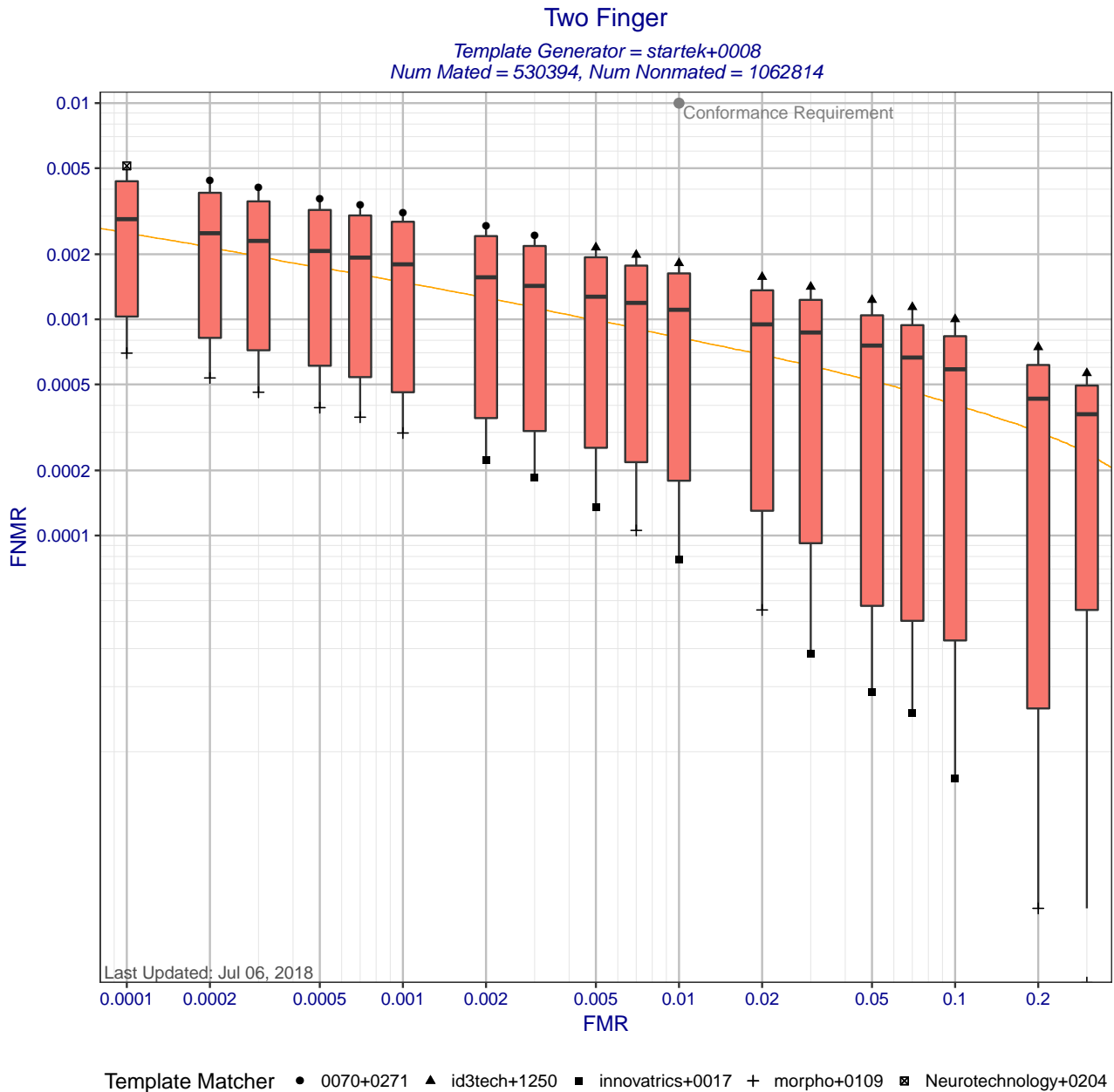
Figure 6: Two Finger DET statistics for template generator startek+0008. Each box shows the distribution of FNMRs at a fixed FMR across different matchers. The whisker ends show the minimum and maximum FNMRs. The orange DET curve shows pooled performance when all matchers use templates created by startek+0008. Score-level fusion is achieved by averaging the scores for left and right index fingers.
