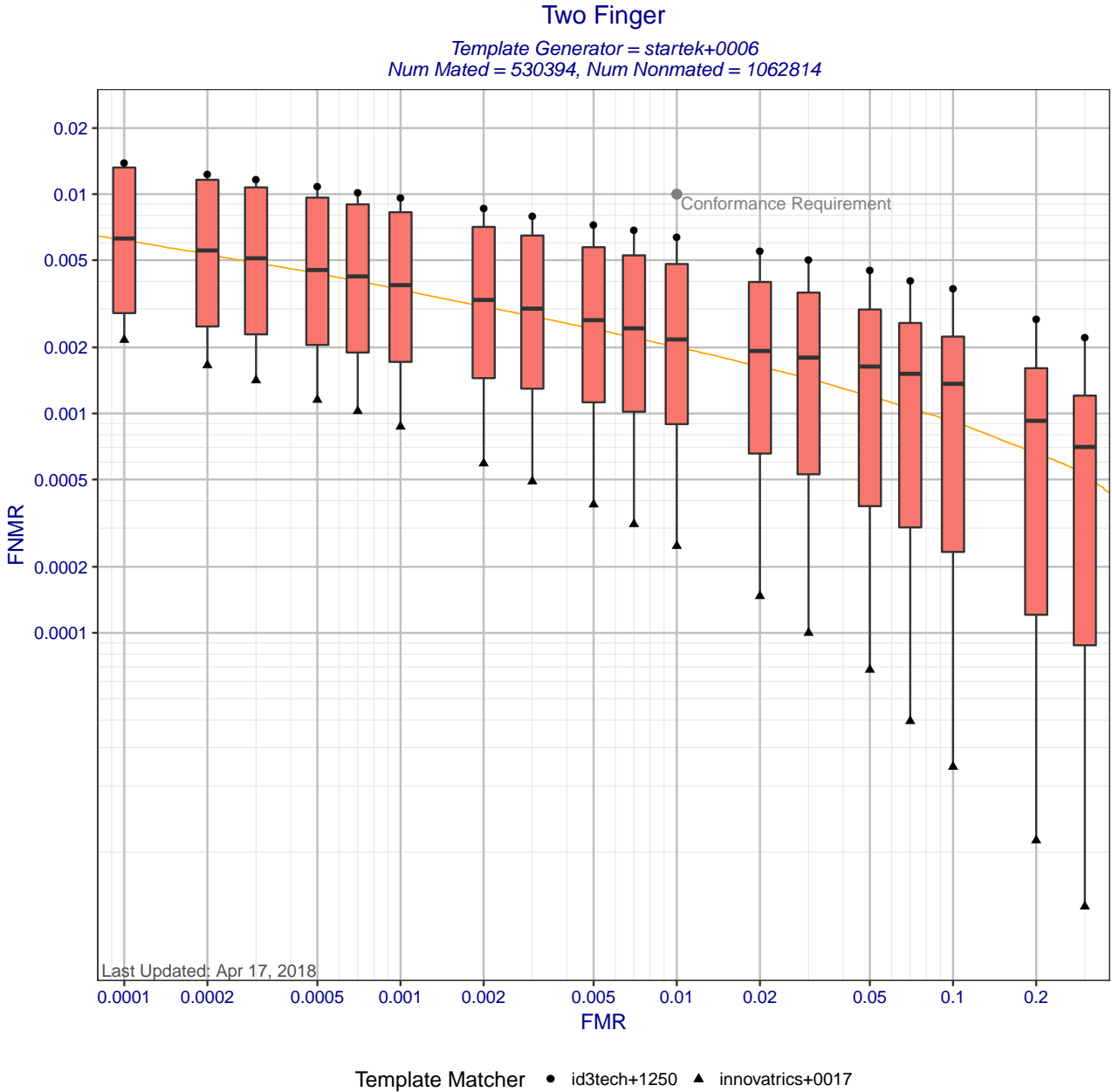
Figure 6: Two Finger DET statistics for template generator startek+0006. Each box shows the distribution of FNMRs at a fixed FMR across different matchers. The whisker ends show the minimum and maximum FNMRs. The orange DET curve shows pooled performance when all matchers use templates created by startek+0006. Score-level fusion is achieved by averaging the scores for left and right index fingers.
