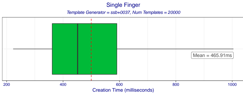
Figure 2: Boxplot of template creation times for template generator ssb+0037. The box edges mark the 10th and 90th percentiles while the whiskers mark the maximum and minimum creation times.
