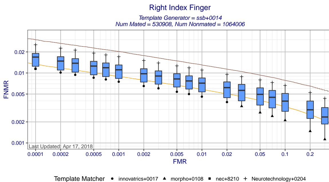
Figure 3: Right Index Finger DET statistics for template generator ssb+0014 . Each box shows the distribution of FNMRs at a fixed FMR across different matchers. The whisker ends show the minimum and maximum FNMRs. The brown curve shows the DET curve when the matcher and template generators were submitted by the same participant. The orange DET curve shows pooled performance when all matchers use templates created by ssb+0014 .
