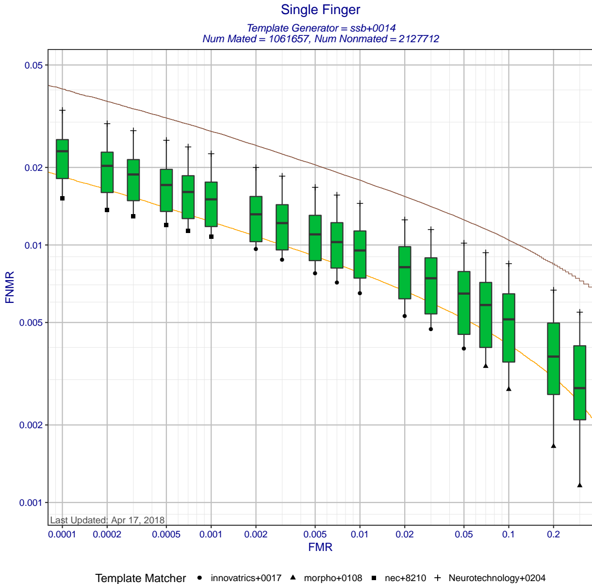
Figure 2: Single finger DET statistics for template generator ssb+0014 . Each box shows the distribution of FNMRs at a fixed FMR across different matchers. The whisker ends show the minimum and maximum FNMRs. The brown curve shows the DET curve when the matcher and template generators were submitted by the same participant. The orange DET curve shows pooled performance when all matchers compare templates created by ssb+0014 .
