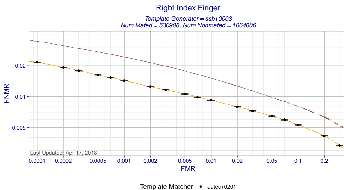
Figure 3: Right Index Finger DET statistics for template generator ssb+0003 . Each box shows the distribution of FNMRs at a fixed FMR across different matchers. The whisker ends show the minimum and maximum FNMRs. The brown curve shows the DET curve when the matcher and template generators were submitted by the same participant. The orange DET curve shows pooled performance when all matchers use templates created by ssb+0003 .
