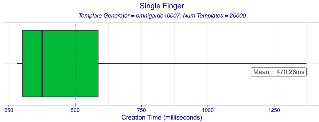
Figure 2: Boxplot of template creation times for template generator omnigarde+0007. The box edges mark the 10th and 90th percentiles while the whiskers mark the maximum and minimum creation times.
