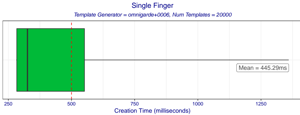
Figure 2: Boxplot of template creation times for template generator omnigarde+0006. The box edges mark the 10th and 90th percentiles while the whiskers mark the maximum and minimum creation times.
