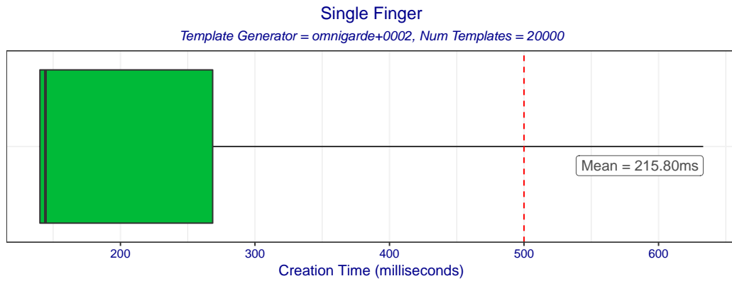
Figure 2: Boxplot of template creation times for template generator omnigarde+0002. The box edges mark the 10th and 90th percentiles while the whiskers mark the maximum and minimum creation times.
