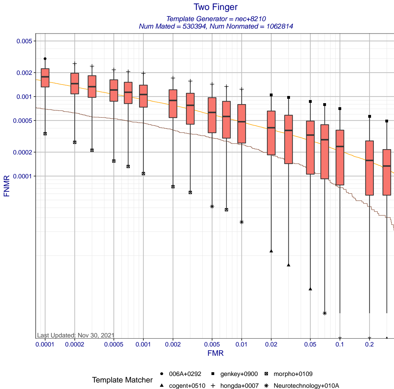
Figure 6: Two Finger DET statistics for template generator nec+8210. Each box shows the distribution of FNMRs at a fixed FMR across different matchers. The whisker ends show the minimum and maximum FNMRs. The brown curve shows the DET curve when the matcher and template generators were submitted by the same participant. The orange DET curve shows pooled performance when all matchers use templates created by nec+8210. Score-level fusion is achieved by averaging the scores for left and right index fingers.
