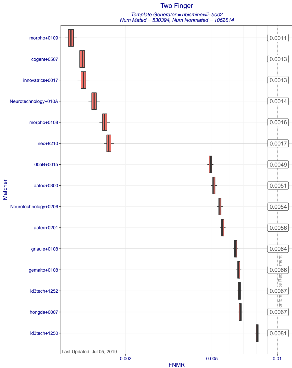
Figure 7: Two Finger FNMR at FMR=0.01 when different matchers compare templates created by template generator nbisminexiii+5002. Each box represents uncertainty about the true FNMR. The box edges mark the 50% confidence intervals while the whiskers mark the 90% confidence intervals. The numbers on the right show the actual computed FNMRs. Score-level fusion is achieved by averaging the scores for left and right index fingers.
