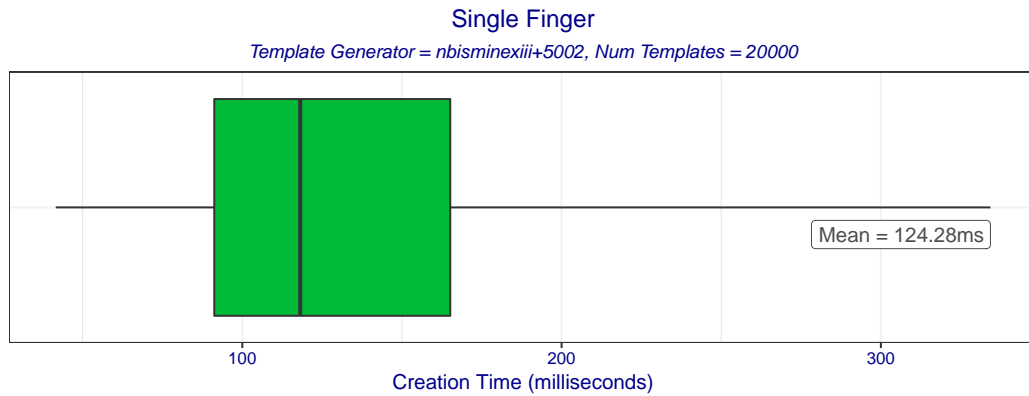
Figure 8: Boxplot of template creation times for template generator nbisminexiii+5002. The box edges mark the 10th and 90th percentiles while the whiskers mark the maximum and minimum creation times.
