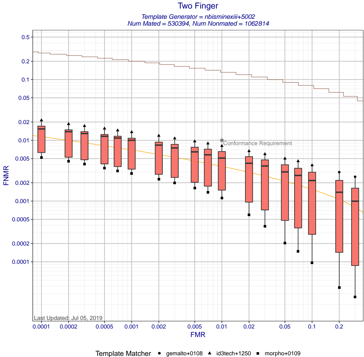
Figure 6: Two Finger DET statistics for template generator nbisminexiii+5002. Each box shows the distribution of FNMRs at a fixed FMR across different matchers. The whisker ends show the minimum and maximum FNMRs. The brown curve shows the DET curve when the matcher and template generators were submitted by the same participant. The orange DET curve shows pooled performance when all matchers use templates created by nbisminexiii+5002. Score-level fusion is achieved by averaging the scores for left and right index fingers.
