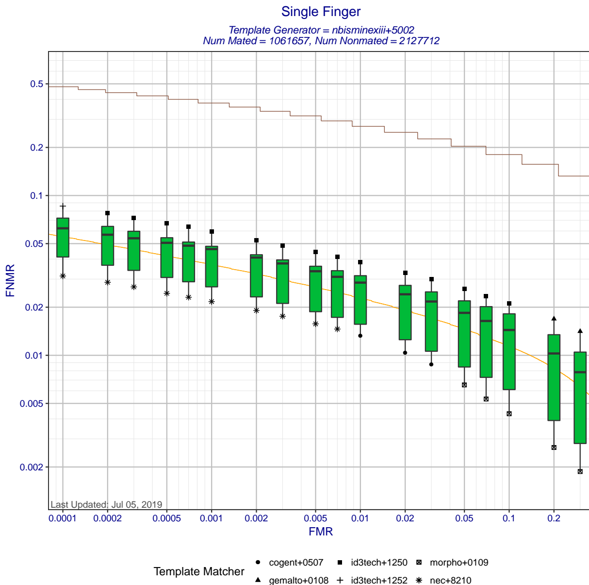
Figure 2: Single finger DET statistics for template generator nbisminexiii+5002. Each box shows the distribution of FNMRs at a fixed FMR across different matchers. The whisker ends show the minimum and maximum FNMRs. The brown curve shows the DET curve when the matcher and template generators were submitted by the same participant. The orange DET curve shows pooled performance when all matchers compare templates created by nbisminexiii+5002.
