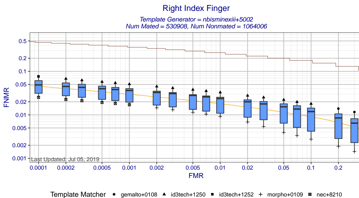
Figure 3: Right Index Finger DET statistics for template generator nbisminexiii+5002. Each box shows the distribution of FNMRs at a fixed FMR across different matchers. The whisker ends show the minimum and maximum FNMRs. The brown curve shows the DET curve when the matcher and template generators were submitted by the same participant. The orange DET curve shows pooled performance when all matchers use templates created by nbisminexiii+5002.
