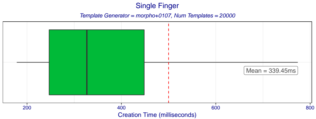
Figure 8: Boxplot of template creation times for template generator morpho+0107. The box edges mark the 10th and 90th percentiles while the whiskers mark the maximum and minimum creation times.
