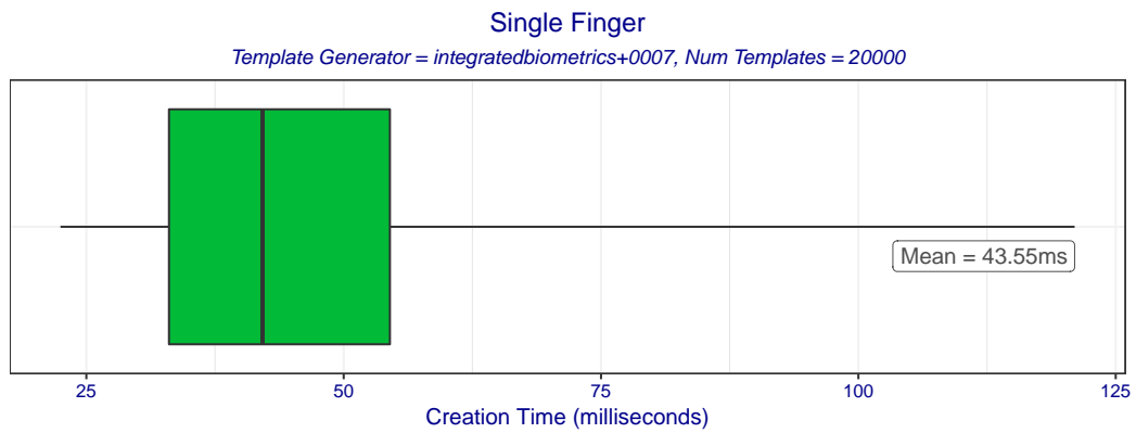
Figure 2: Boxplot of template creation times for template generator integratedbiometrics+0007. The box edges mark the 10th and 90th percentiles while the whiskers mark the maximum and minimum creation times.
