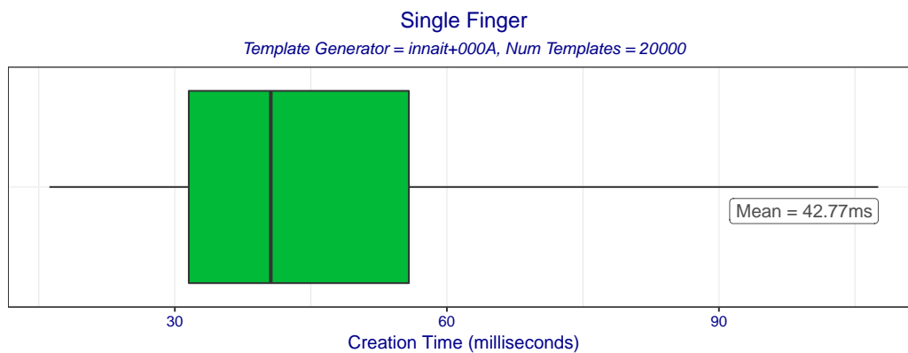
Figure 2: Boxplot of template creation times for template generator innait+000A. The box edges mark the 10th and 90th percentiles while the whiskers mark the maximum and minimum creation times.
