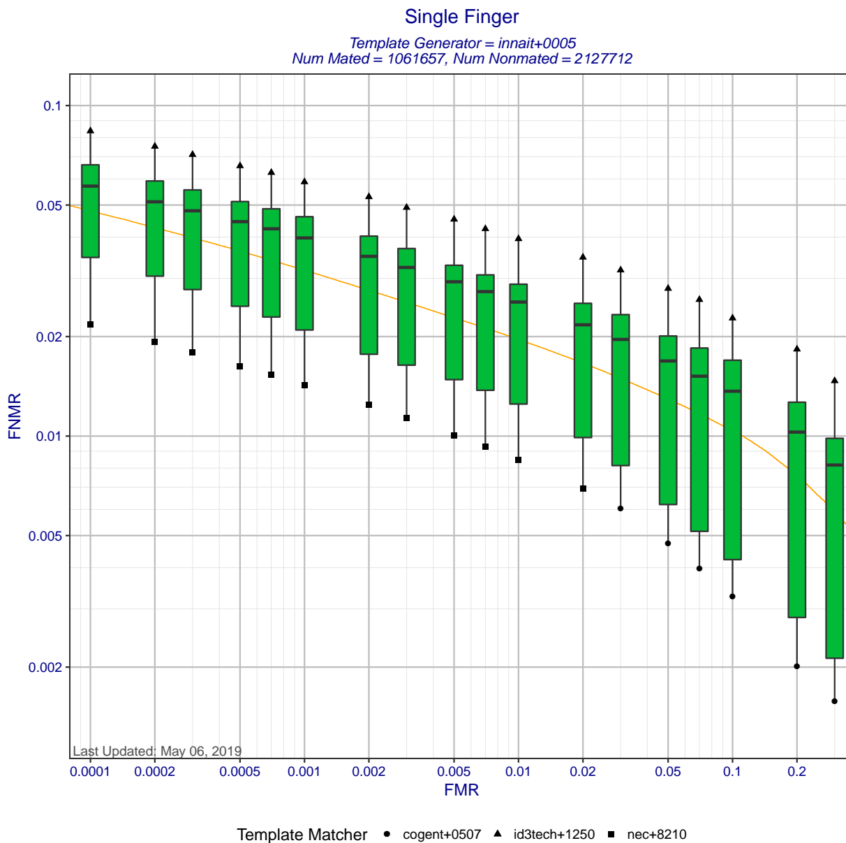
Figure 2: Single finger DET statistics for template generator innait+0005. Each box shows the distribution of FNMRs at a fixed FMR across different matchers. The whisker ends show the minimum and maximum FNMRs. The orange DET curve shows pooled performance when all matchers compare templates created by innait+0005.
