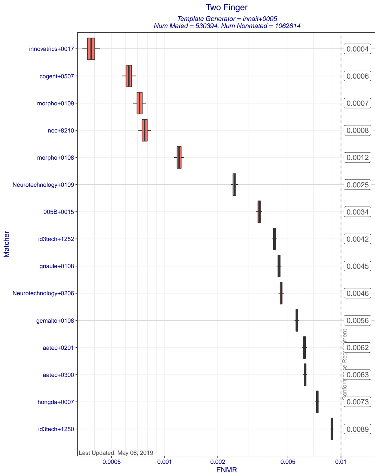
Figure 7: Two Finger FNMR at FMR=0.01 when different matchers compare templates created by template generator innait+0005. Each box represents uncertainty about the true FNMR. The box edges mark the 50% confidence intervals while the whiskers mark the 90% confidence intervals. The numbers on the right show the actual computed FNMRs. Score-level fusion is achieved by averaging the scores for left and right index fingers.
