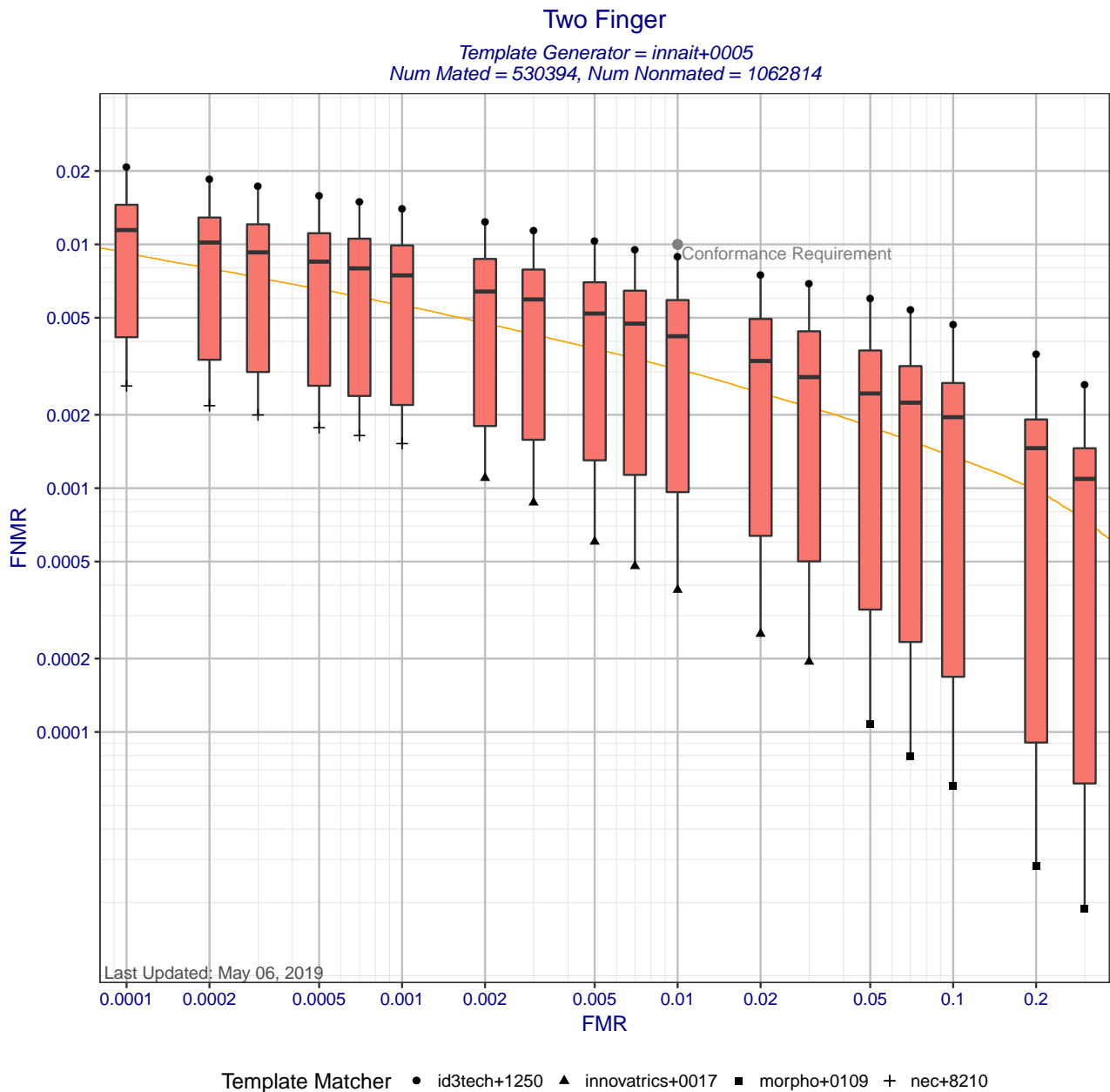
Figure 6: Two Finger DET statistics for template generator innait+0005. Each box shows the distribution of FNMRs at a fixed FMR across different matchers. The whisker ends show the minimum and maximum FNMRs. The orange DET curve shows pooled performance when all matchers use templates created by innait+0005. Score-level fusion is achieved by averaging the scores for left and right index fingers.
