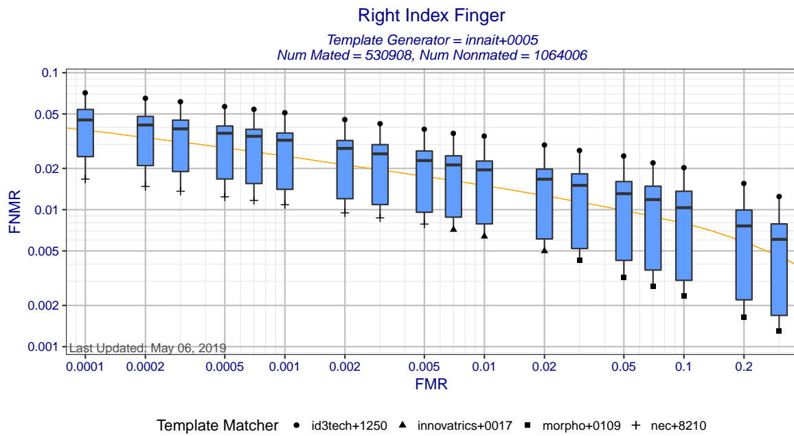
Figure 3: Right Index Finger DET statistics for template generator innait+0005 . Each box shows the distribution of FNMRs at a fixed FMR across different matchers. The whisker ends show the minimum and maximum FNMRs. The orange DET curve shows pooled performance when all matchers use templates created by innait+0005 .
