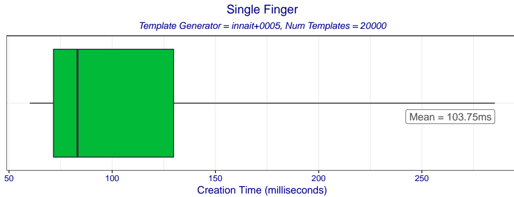
Figure 8: Boxplot of template creation times for template generator innait+0005. The box edges mark the 10th and 90th percentiles while the whiskers mark the maximum and minimum creation times.
