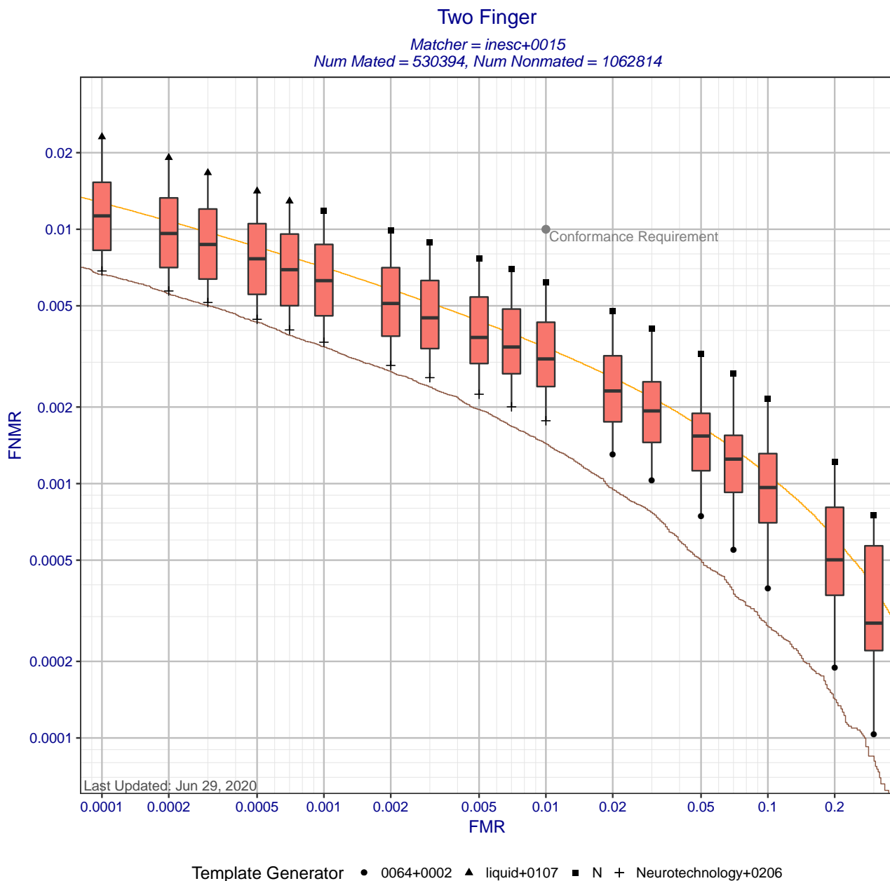
Figure 7: Two finger DET statistics for matcher inesc+0015. Each box shows the distribution of FNMRs at a fixed FMR across all MINEX III compliant template generators. The whisker ends show the minimum and maximum FNMRs. The orange DET curve shows pooled performance against all template generators. Score-level fusion is achieved by averaging the scores for left and right index fingers.
