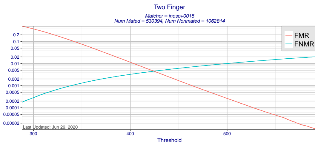
Figure 12: Two finger FMR and FNMR as a function of score threshold for matcher inesc+0015 using templates created by all MINEX III compliant template generators. Score-level fusion is achieved by averaging scores for the left and right index fingers.
