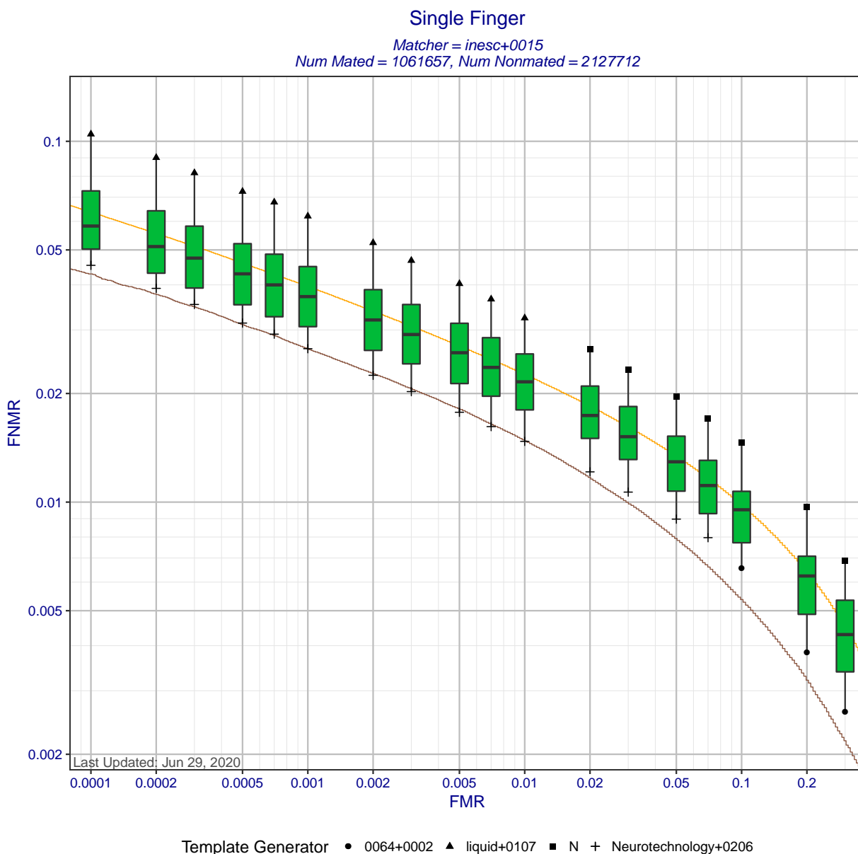
Figure 2: Single finger DET statistics for matcher inesc+0015. Each box shows the distribution of FNMRs at a fixed FMR across all MINEX III compliant template generators. The ends of the whiskers show the minimum and maximum FNMRs. The orange DET curve shows pooled performance against all template generators.
