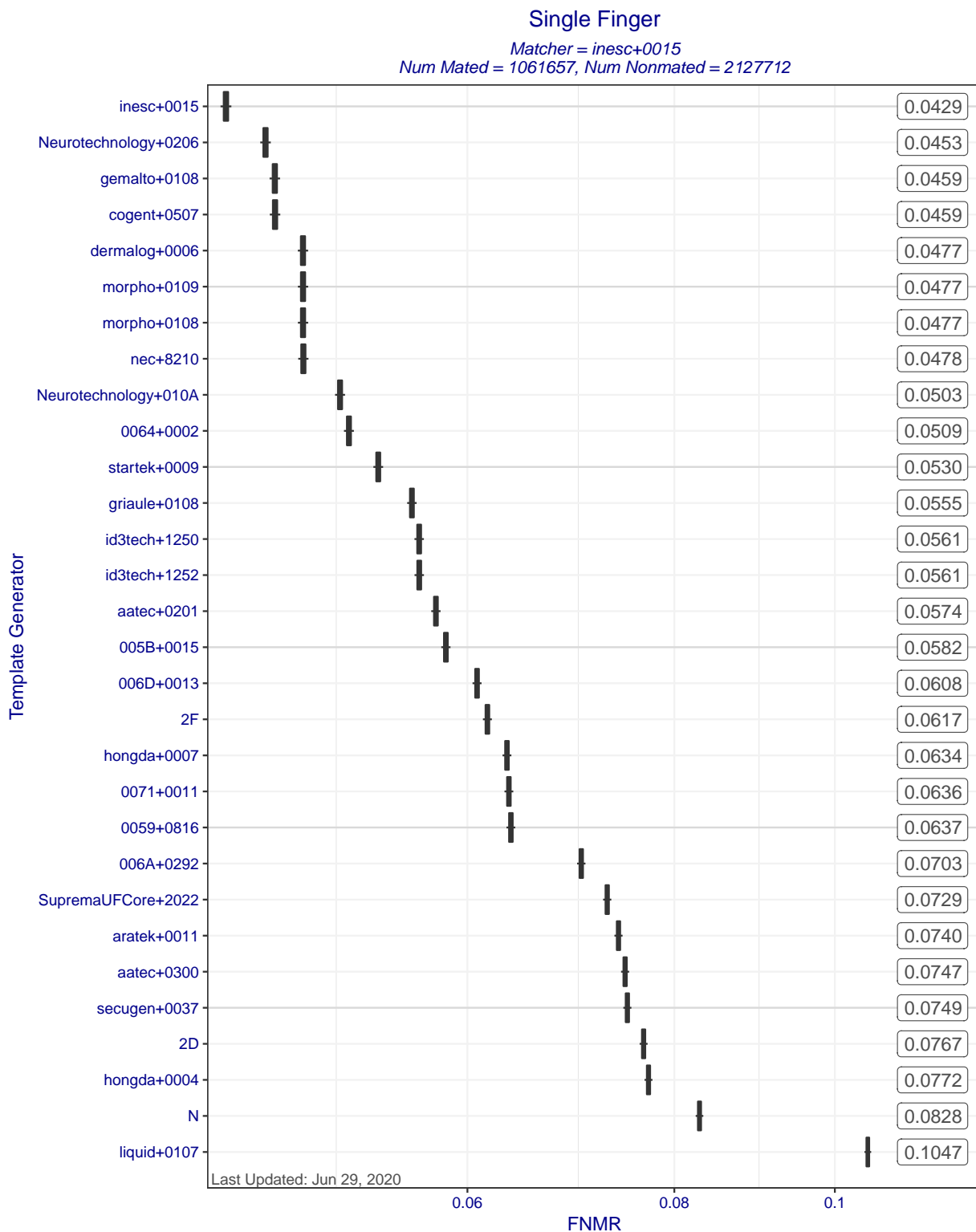
Figure 5: Single finger FNMRs at FMR = 0.0001 when matcher inesc+0015 compares templates created by different template generators. The ends of the whiskers show the minimum and maximum FNMRs. Each box represents uncertainty about the true FNMR. The box edges mark the 50% confidence intervals while the whiskers mark the 90% confidence intervals. The numbers on the right show the actual computed FNMRs.
