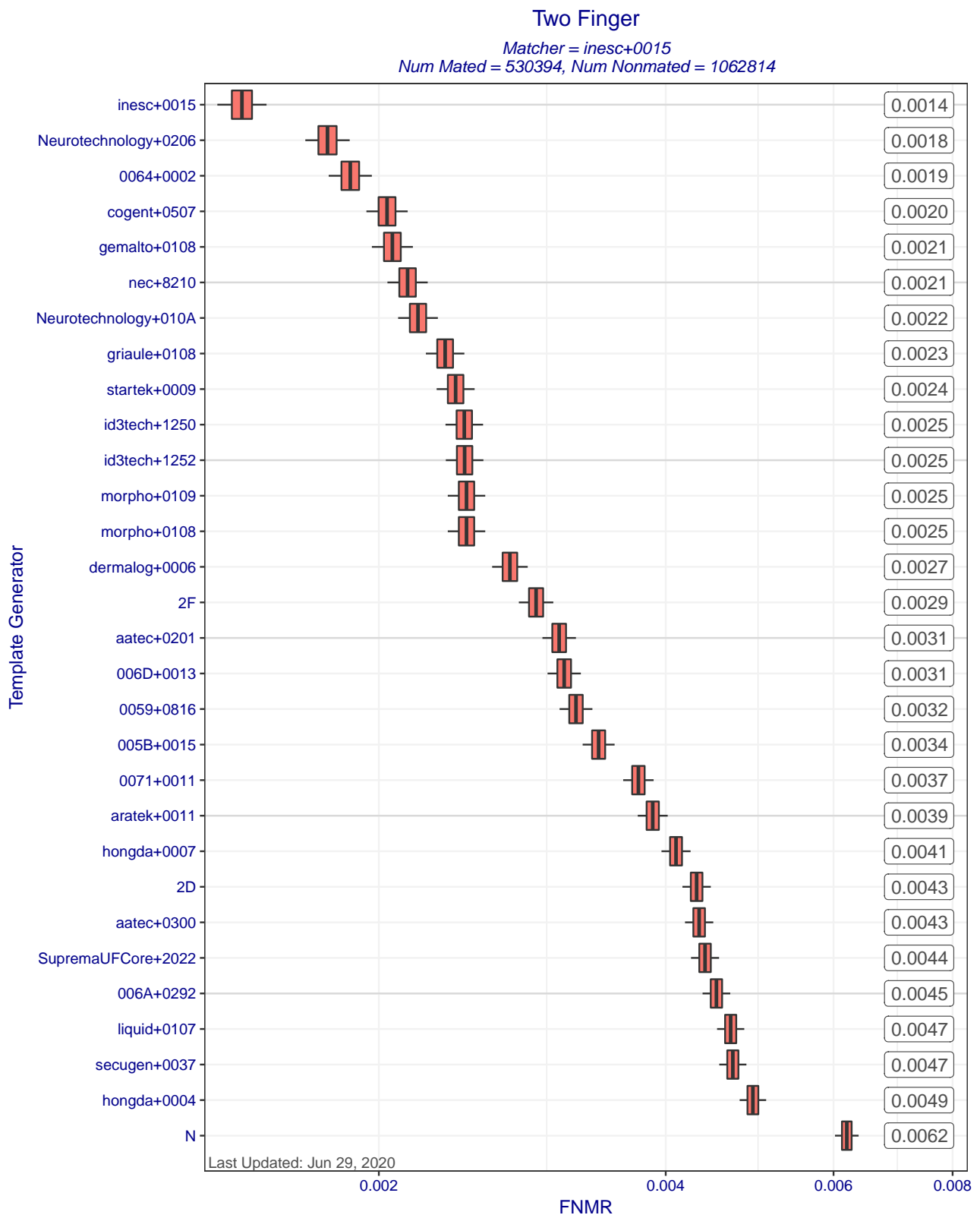
Figure 8: Two finger FNMR at FMR=0.01 when matcher inesc+0015 compares templates created by different template generators. Each box represents uncertainty about the true FNMR. The box edges mark the 50% confidence intervals while the whiskers mark the 90% confidence intervals. The numbers on the right show the actual computed FNMRs. Score-level fusion is achieved by averaging the scores for left and right index fingers.
