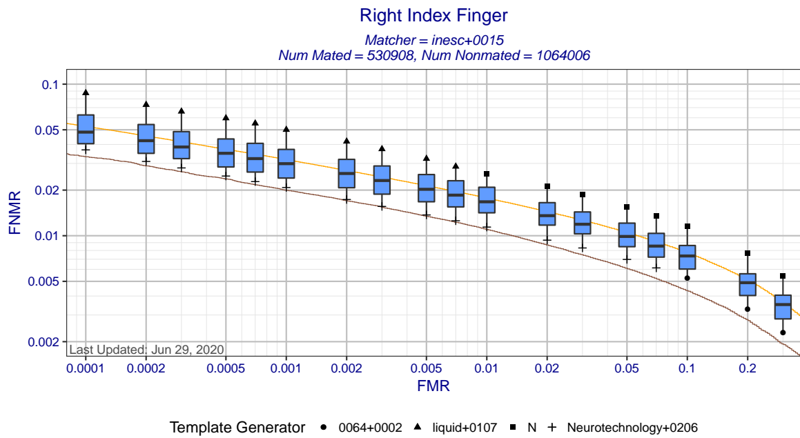
Figure 3: Right index finger DET statistics for matcher inesc+0015. Each box shows the distribution of FNMR at a fixed FMR across all MINEX III compliant template generators. The ends of the whiskers show the minimum and maximum FNMRs. The orange DET curve shows pooled performance against all template generators.
