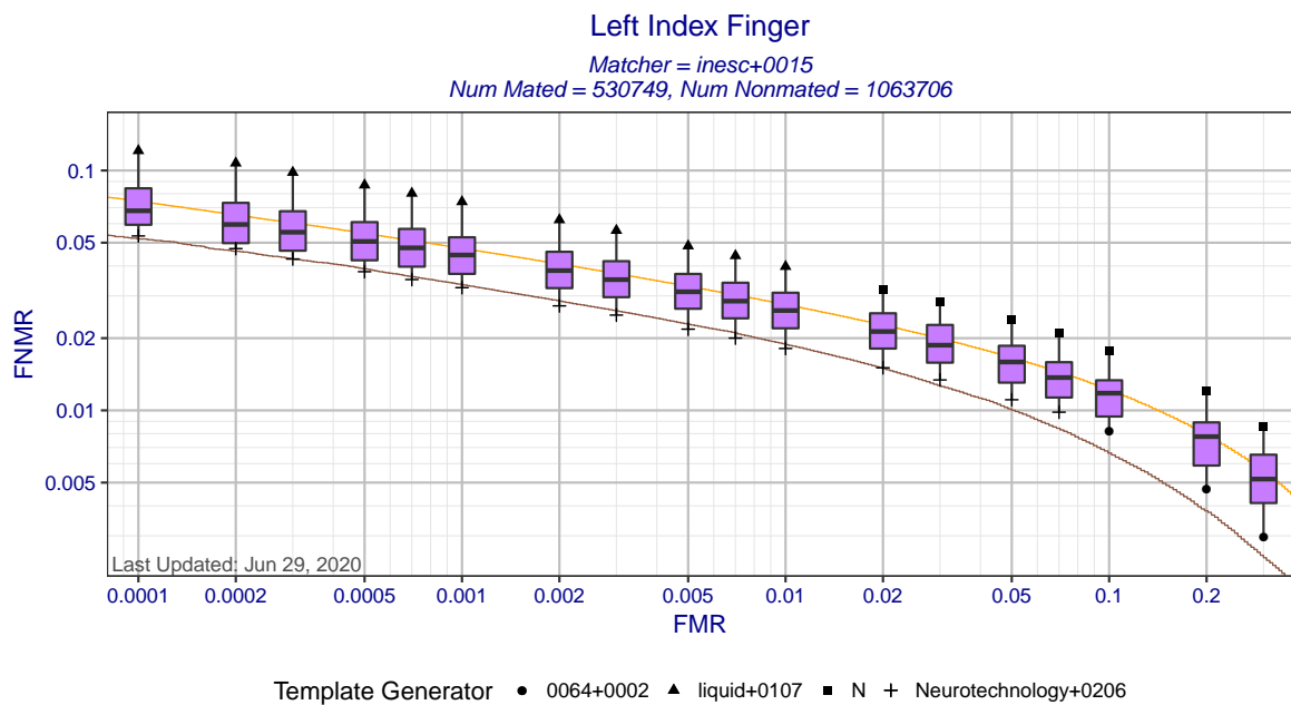
Figure 4: Left index finger DET statistics for matcher inesc+0015. Each box shows the distribution of FNMRs at a fixed FMR across all MINEX III compliant template generators. The ends of whiskers show the minimum and maximum FNMRs. The orange DET curve shows pooled performance against all template generators.
