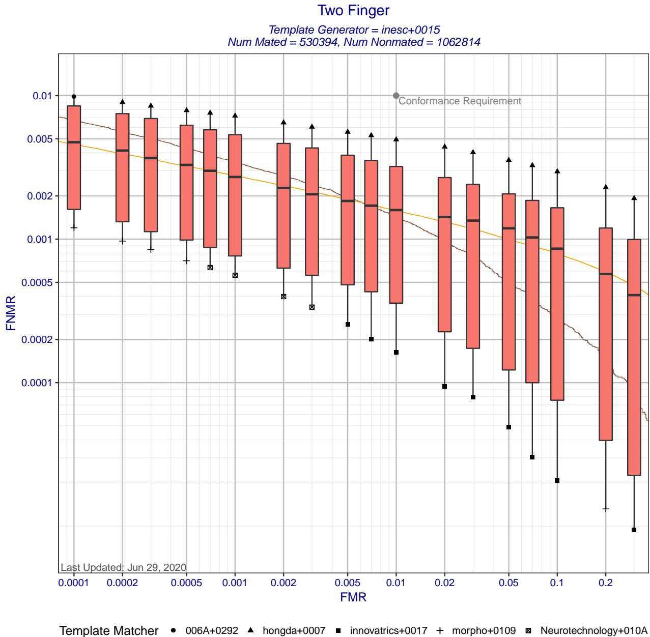
Figure 6: Two Finger DET statistics for template generator inesc+0015. Each box shows the distribution of FNMRs at a fixed FMR across different matchers. The whisker ends show the minimum and maximum FNMRs. The brown curve shows the DET curve when the matcher and template generators were submitted by the same participant. The orange DET curve shows pooled performance when all matchers use templates created by inesc+0015. Score-level fusion is achieved by averaging the scores for left and right index fingers.
