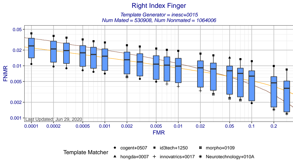
Figure 3: Right Index Finger DET statistics for template generator inesc+0015. Each box shows the distribution of FNMRs at a fixed FMR across different matchers. The whisker ends show the minimum and maximum FNMRs. The brown curve shows the DET curve when the matcher and template generators were submitted by the same participant. The orange DET curve shows pooled performance when all matchers use templates created by inesc+0015.
