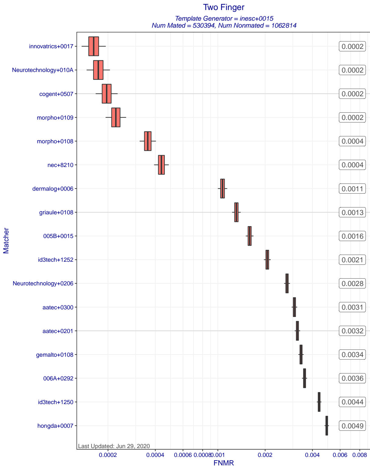
Figure 7: Two Finger FNMR at FMR=0.01 when different matchers compare templates created by template generator inesc+0015. Each box represents uncertainty about the true FNMR. The box edges mark the 50% confidence intervals while the whiskers mark the 90% confidence intervals. The numbers on the right show the actual computed FNMRs. Score-level fusion is achieved by averaging the scores for left and right index fingers.
