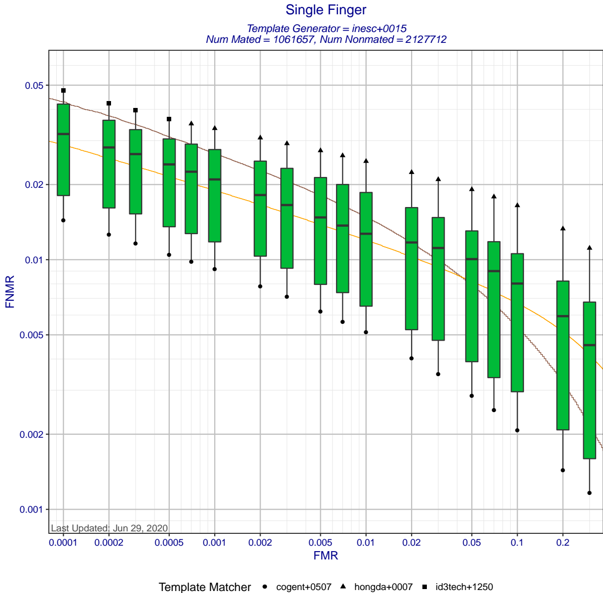
Figure 2: Single finger DET statistics for template generator inesc+0015. Each box shows the distribution of FNMRs at a fixed FMR across different matchers. The whisker ends show the minimum and maximum FNMRs. The brown curve shows the DET curve when the matcher and template generators were submitted by the same participant. The orange DET curve shows pooled performance when all matchers compare templates created by inesc+0015.
