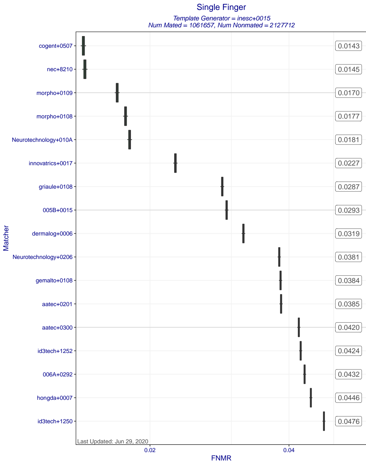
Figure 5: Single Finger FNMRs at FMR=0.0001 when MINEX III compliant matchers compare templates created by template generator inesc+0015. Each box represents uncertainty about the true FNMR. The box edges mark the 50% confidence intervals while the whiskers mark the 90% confidence intervals. The numbers on the right show the actual computed FNMRs.
