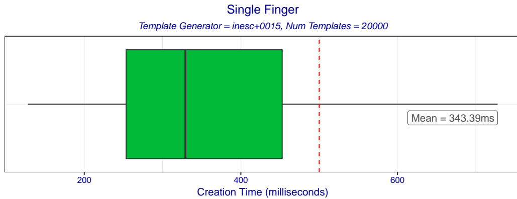
Figure 8: Boxplot of template creation times for template generator inesc+0015 . The box edges mark the 10th and 90th percentiles while the whiskers mark the maximum and minimum creation times.
