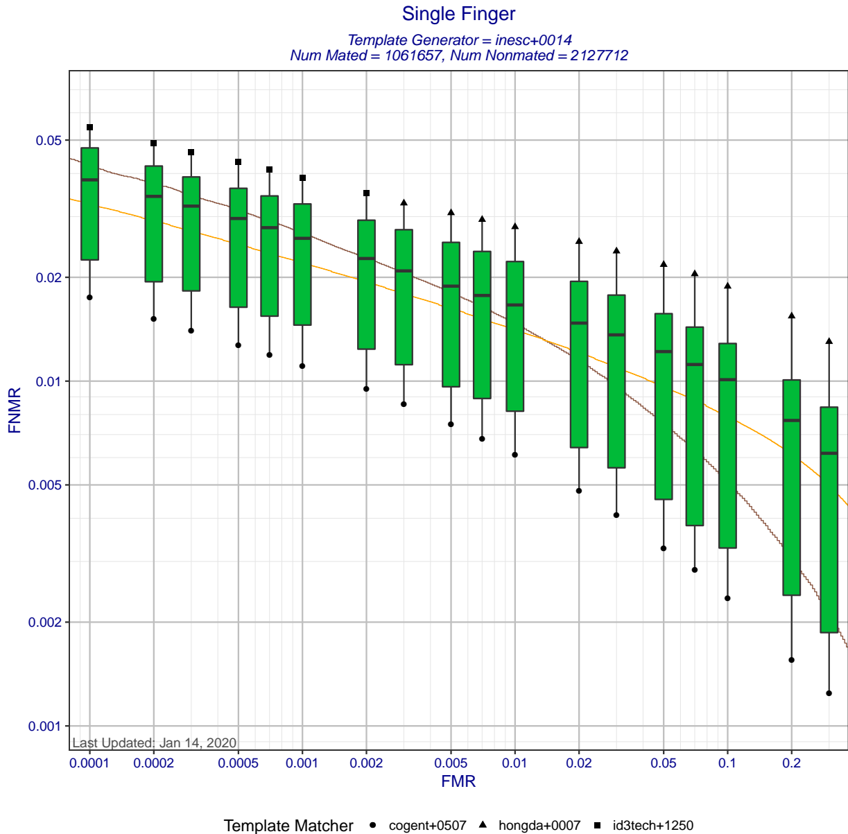
Figure 2: Single finger DET statistics for template generator inesc+0014. Each box shows the distribution of FNMRs at a fixed FMR across different matchers. The whisker ends show the minimum and maximum FNMRs. The brown curve shows the DET curve when the matcher and template generators were submitted by the same participant. The orange DET curve shows pooled performance when all matchers compare templates created by inesc+0014.
