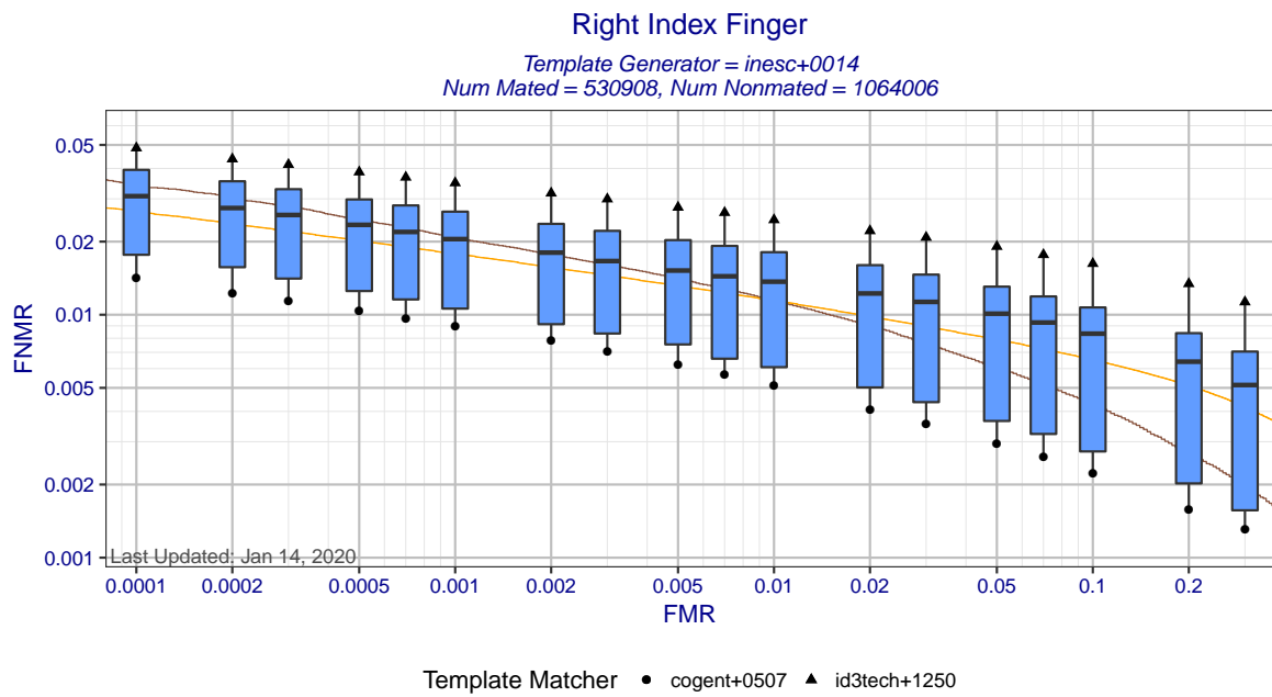
Figure 3: Right Index Finger DET statistics for template generator inesc+0014. Each box shows the distribution of FNMRs at a fixed FMR across different matchers. The whisker ends show the minimum and maximum FNMRs. The brown curve shows the DET curve when the matcher and template generators were submitted by the same participant. The orange DET curve shows pooled performance when all matchers use templates created by inesc+0014.
