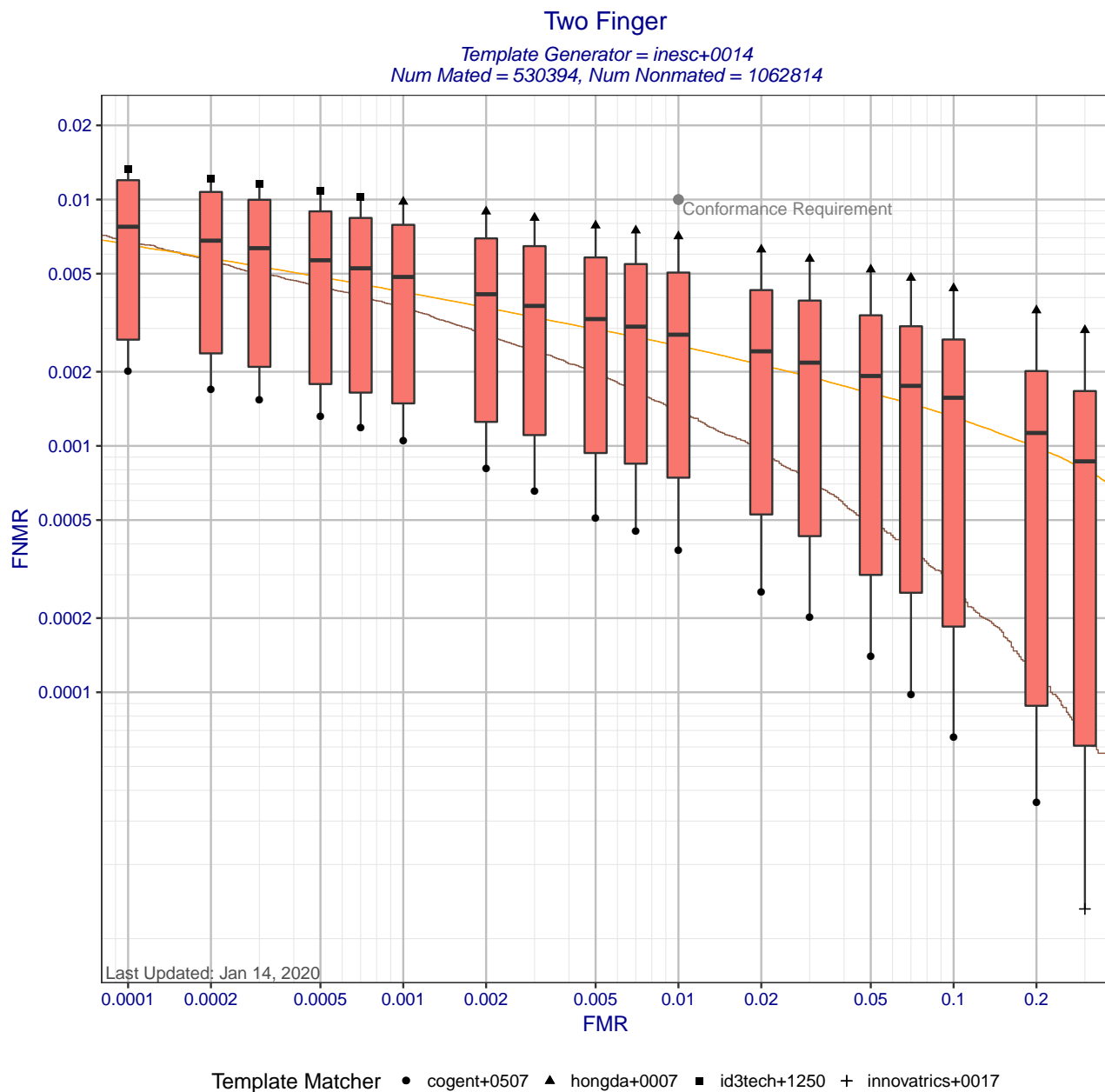
Figure 6: Two Finger DET statistics for template generator inesc+0014. Each box shows the distribution of FNMRs at a fixed FMR across different matchers. The whisker ends show the minimum and maximum FNMRs. The brown curve shows the DET curve when the matcher and template generators were submitted by the same participant. The orange DET curve shows pooled performance when all matchers use templates created by inesc+0014. Score-level fusion is achieved by averaging the scores for left and right index fingers.
