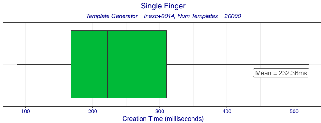
Figure 8: Boxplot of template creation times for template generator inesc+0014. The box edges mark the 10th and 90th percentiles while the whiskers mark the maximum and minimum creation times.
