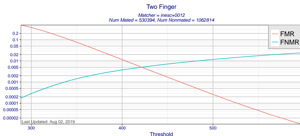
Figure 12: Two finger FMR and FNMR as a function of score threshold for matcher inesc+0012 using templates created by all MINEX III compliant template generators. Score-level fusion is achieved by averaging scores for the left and right index fingers.
