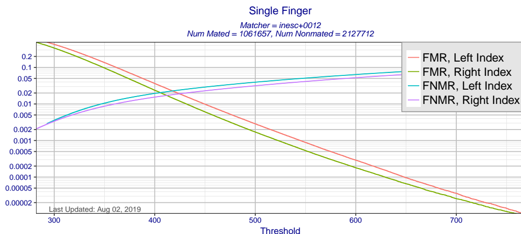
Figure 11: Single finger FMR and FNMR as a function of score threshold for matcher inesc+0012 using templates created by all MINEX III compliant template generators. Separate curves are presented for left and right index fingers.
