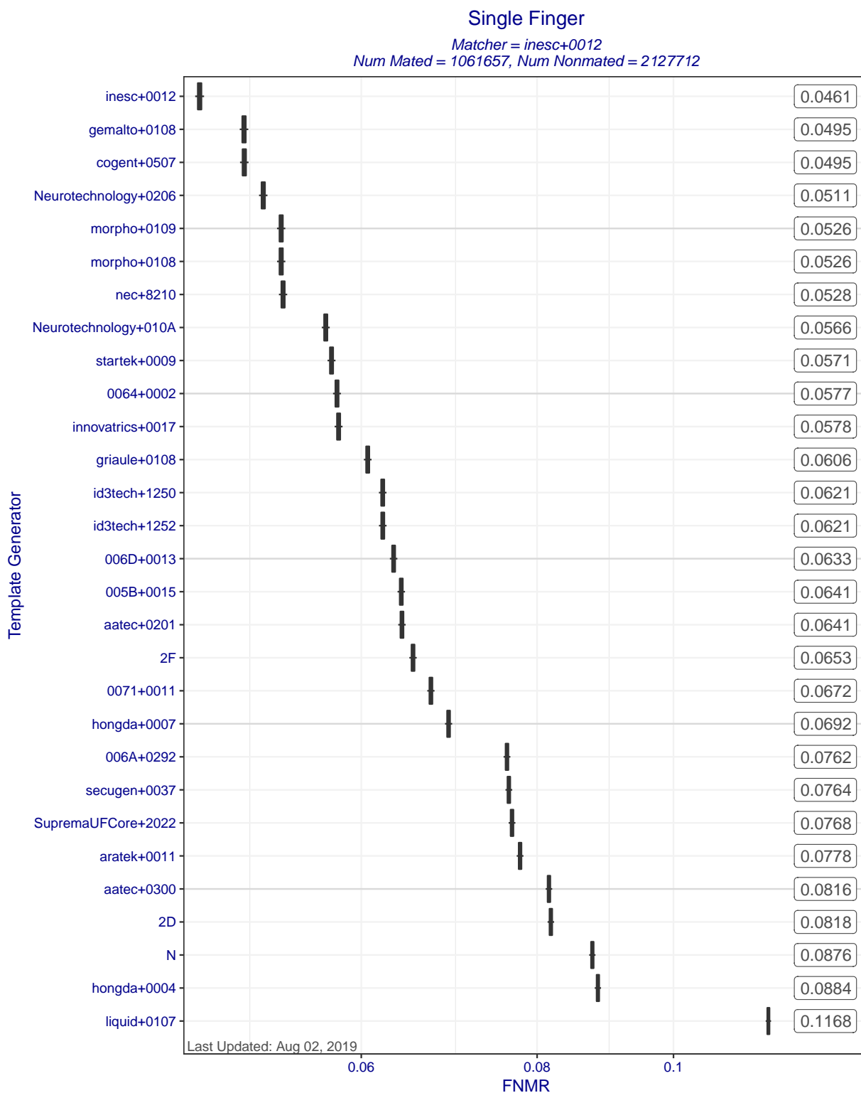
Figure 5: Single finger FNMRs at FMR = 0.0001 when matcher inesc+0012 compares templates created by different template generators. The ends of the whiskers show the minimum and maximum FNMRs. Each box represents uncertainty about the true FNMR. The box edges mark the 50% confidence intervals while the whiskers mark the 90% confidence intervals. The numbers on the right show the actual computed FNMRs.
