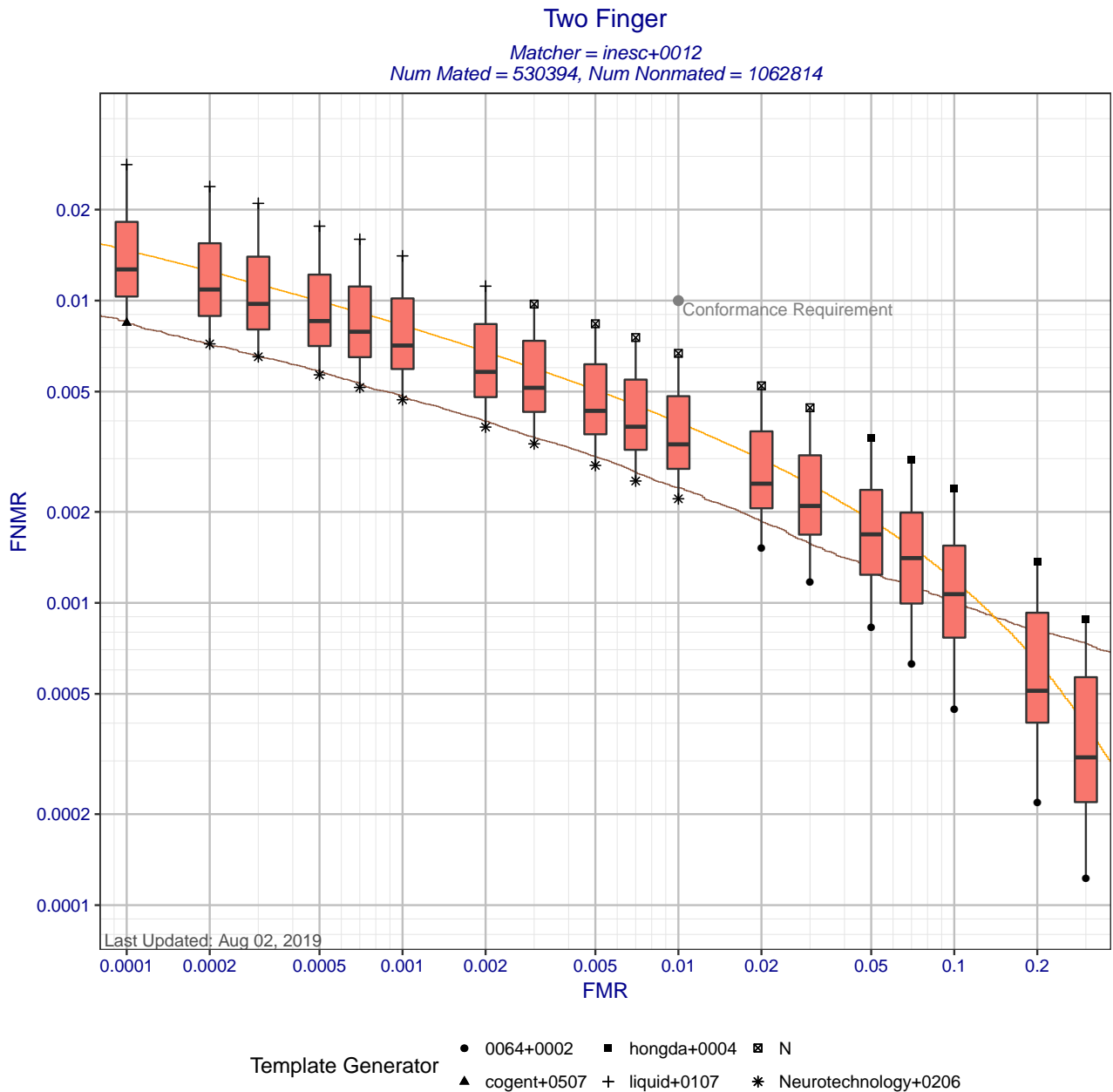
Figure 7: Two finger DET statistics for matcher inesc+0012. Each box shows the distribution of FNMRs at a fixed FMR across all MINEX III compliant template generators. The whisker ends show the minimum and maximum FNMRs. The orange DET curve shows pooled performance against all template generators. Score-level fusion is achieved by averaging the scores for left and right index fingers.
