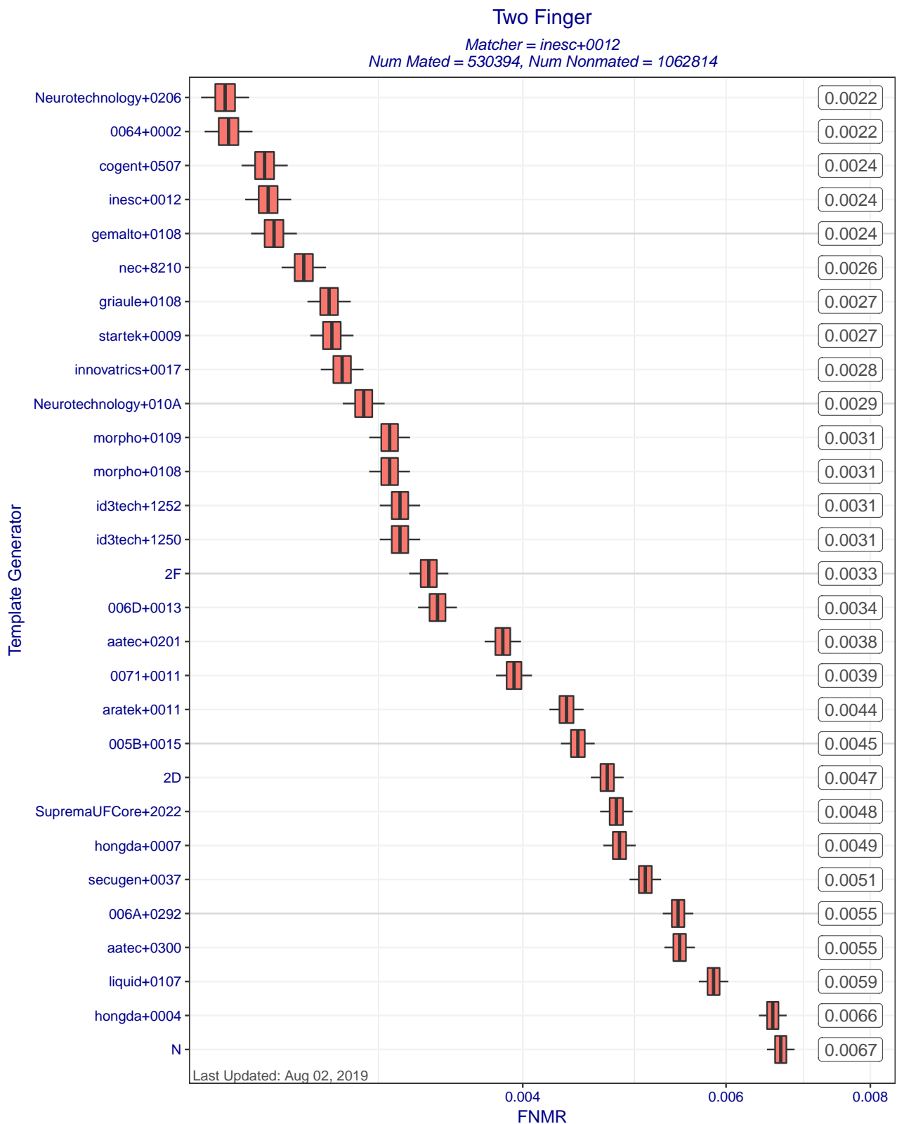
Figure 8: Two finger FNMR at FMR=0.01 when matcher inesc+0012 compares templates created by different template generators. Each box represents uncertainty about the true FNMR. The box edges mark the 50% confidence intervals while the whiskers mark the 90% confidence intervals. The numbers on the right show the actual computed FNMRs. Score-level fusion is achieved by averaging the scores for left and right index fingers.
