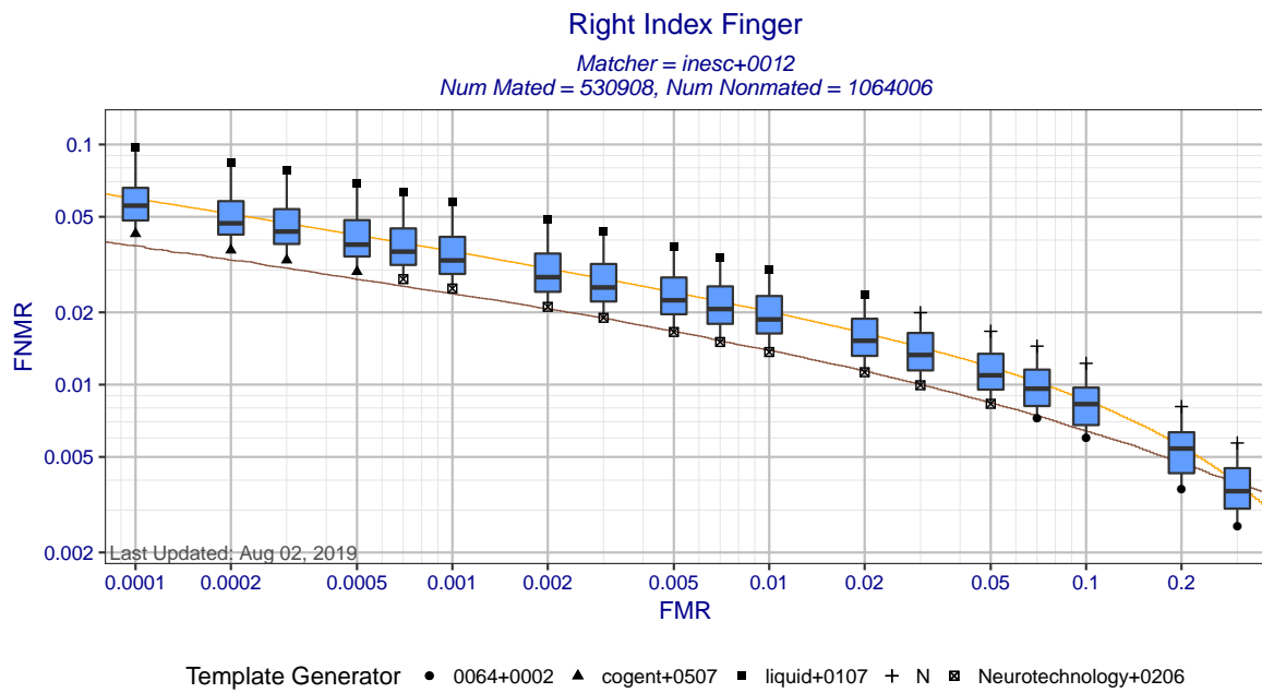
Figure 3: Right index finger DET statistics for matcher inesc+0012. Each box shows the distribution of FNMR at a fixed FMR across all MINEX III compliant template generators. The ends of the whiskers show the minimum and maximum FNMRs. The orange DET curve shows pooled performance against all template generators.
