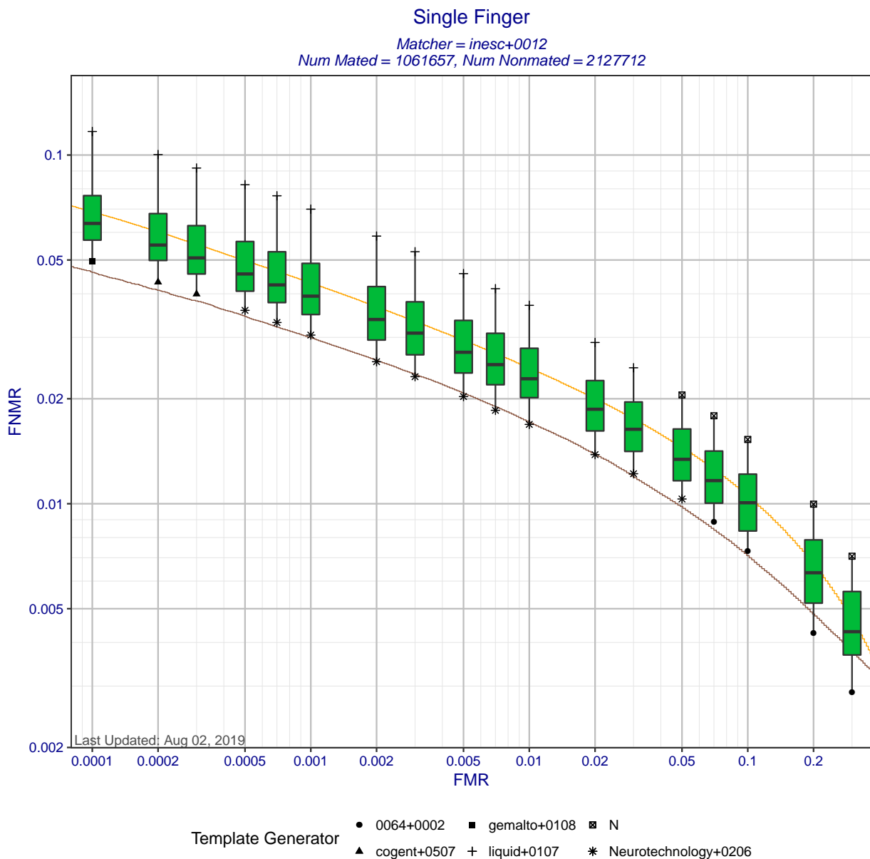
Figure 2: Single finger DET statistics for matcher inesc+0012. Each box shows the distribution of FNMRs at a fixed FMR across all MINEX III compliant template generators. The ends of the whiskers show the minimum and maximum FNMRs. The orange DET curve shows pooled performance against all template generators.
