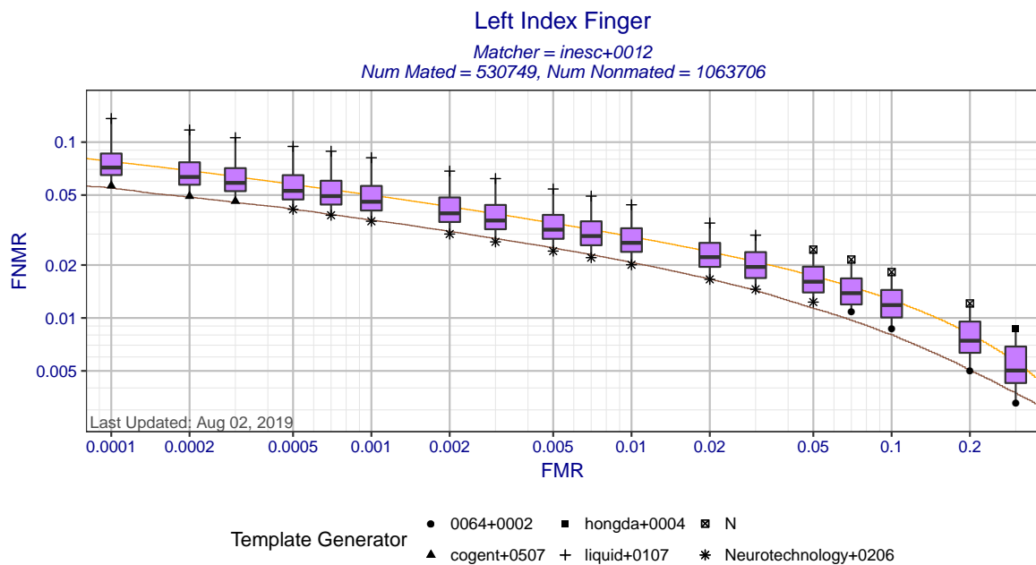
Figure 4: Left index finger DET statistics for matcher inesc+0012. Each box shows the distribution of FNMRs at a fixed FMR across all MINEX III compliant template generators. The ends of whiskers show the minimum and maximum FNMRs. The orange DET curve shows pooled performance against all template generators.
