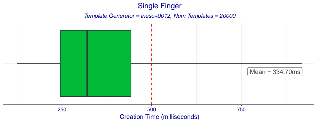
Figure 8: Boxplot of template creation times for template generator inesc+0012 . The box edges mark the 10th and 90th percentiles while the whiskers mark the maximum and minimum creation times.
