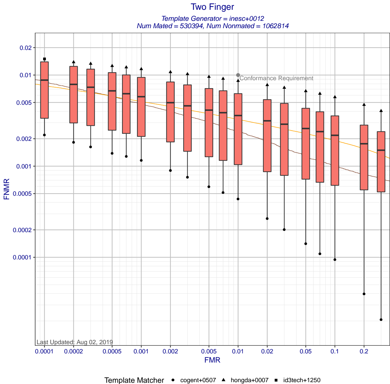
Figure 6: Two Finger DET statistics for template generator inesc+0012. Each box shows the distribution of FNMRs at a fixed FMR across different matchers. The whisker ends show the minimum and maximum FNMRs. The brown curve shows the DET curve when the matcher and template generators were submitted by the same participant. The orange DET curve shows pooled performance when all matchers use templates created by inesc+0012. Score-level fusion is achieved by averaging the scores for left and right index fingers.
