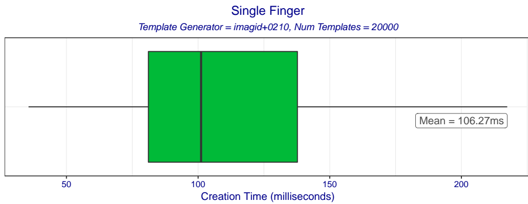
Figure 2: Boxplot of template creation times for template generator imagid+0210. The box edges mark the 10th and 90th percentiles while the whiskers mark the maximum and minimum creation times.
