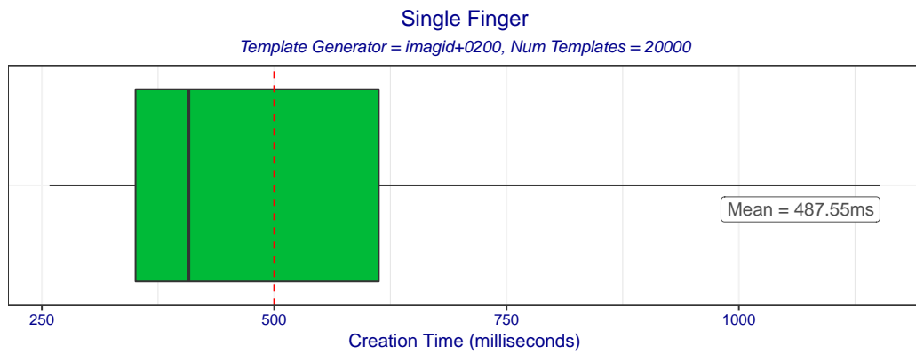
Figure 2: Boxplot of template creation times for template generator imagid+0200. The box edges mark the 10th and 90th percentiles while the whiskers mark the maximum and minimum creation times.
