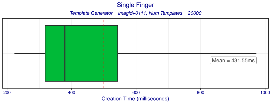
Figure 2: Boxplot of template creation times for template generator imagid+0111. The box edges mark the 10th and 90th percentiles while the whiskers mark the maximum and minimum creation times.
