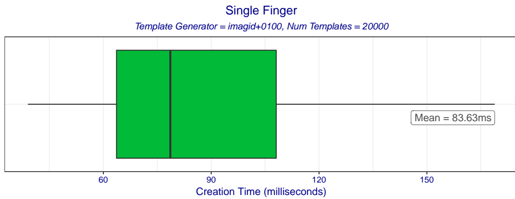
Figure 2: Boxplot of template creation times for template generator imagid+0100. The box edges mark the 10th and 90th percentiles while the whiskers mark the maximum and minimum creation times.
