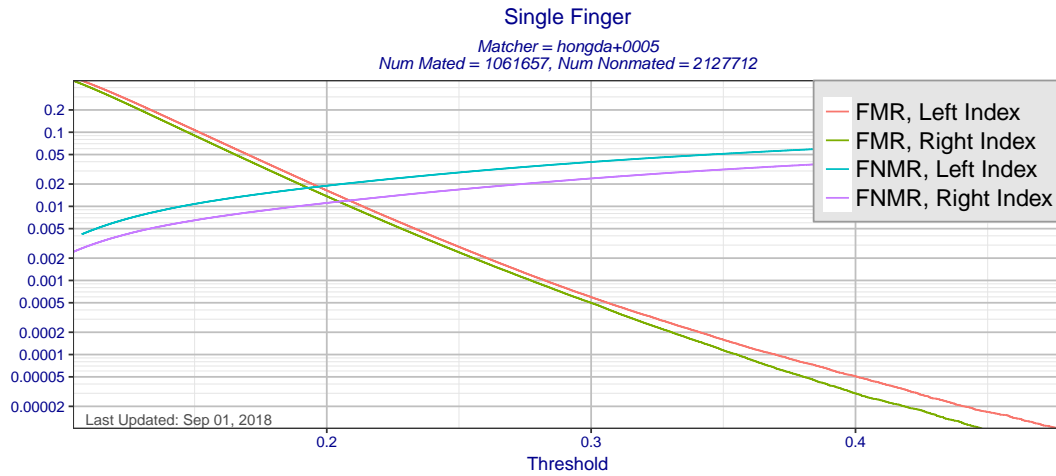
Figure 11: Single finger FMR and FNMR as a function of score threshold for matcher hongda+0005 using templates created by all MINEX III compliant template generators. Separate curves are presented for left and right index fingers.
