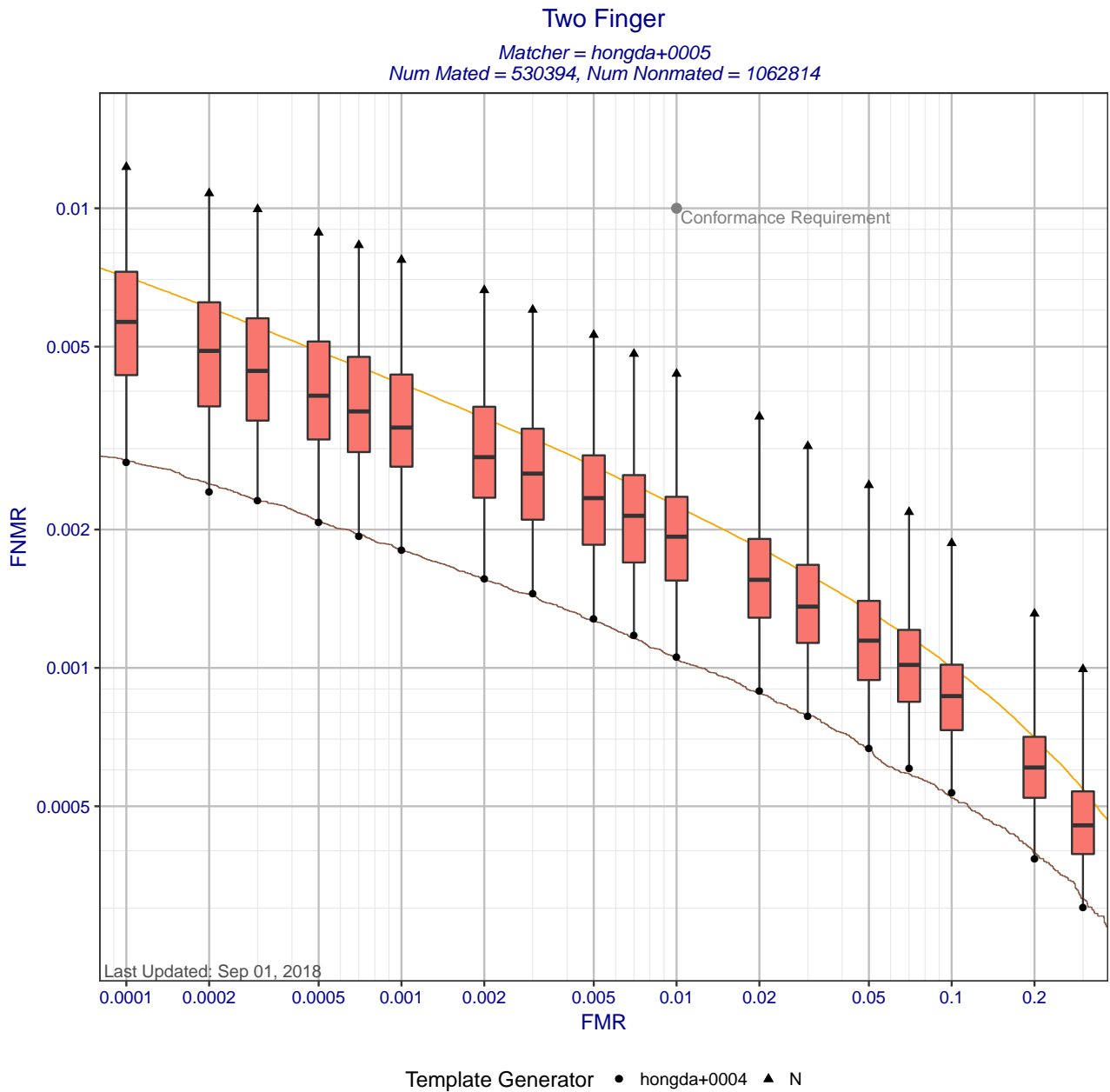
Figure 7: Two finger DET statistics for matcher hongda+0005. Each box shows the distribution of FNMRs at a fixed FMR across all MINEX III compliant template generators. The whisker ends show the minimum and maximum FNMRs. The orange DET curve shows pooled performance against all template generators. Score-level fusion is achieved by averaging the scores for left and right index fingers.
