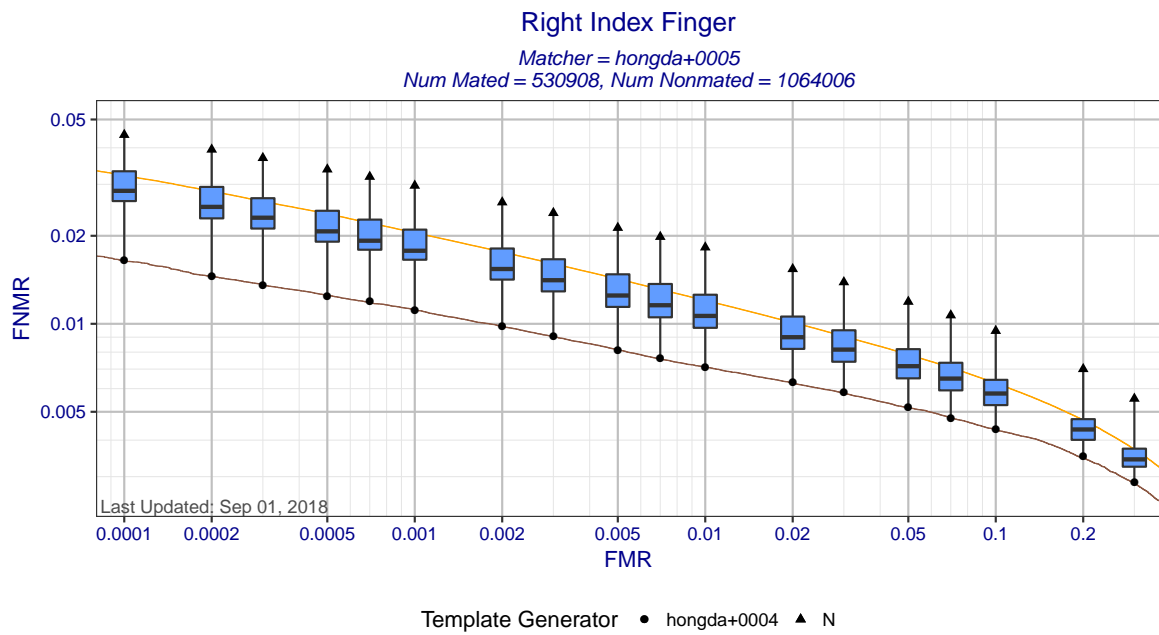
Figure 3: Right index finger DET statistics for matcher hongda+0005. Each box shows the distribution of FNMR at a fixed FMR across all MINEX III compliant template generators. The ends of the whiskers show the minimum and maximum FNMRs. The orange DET curve shows pooled performance against all template generators.
