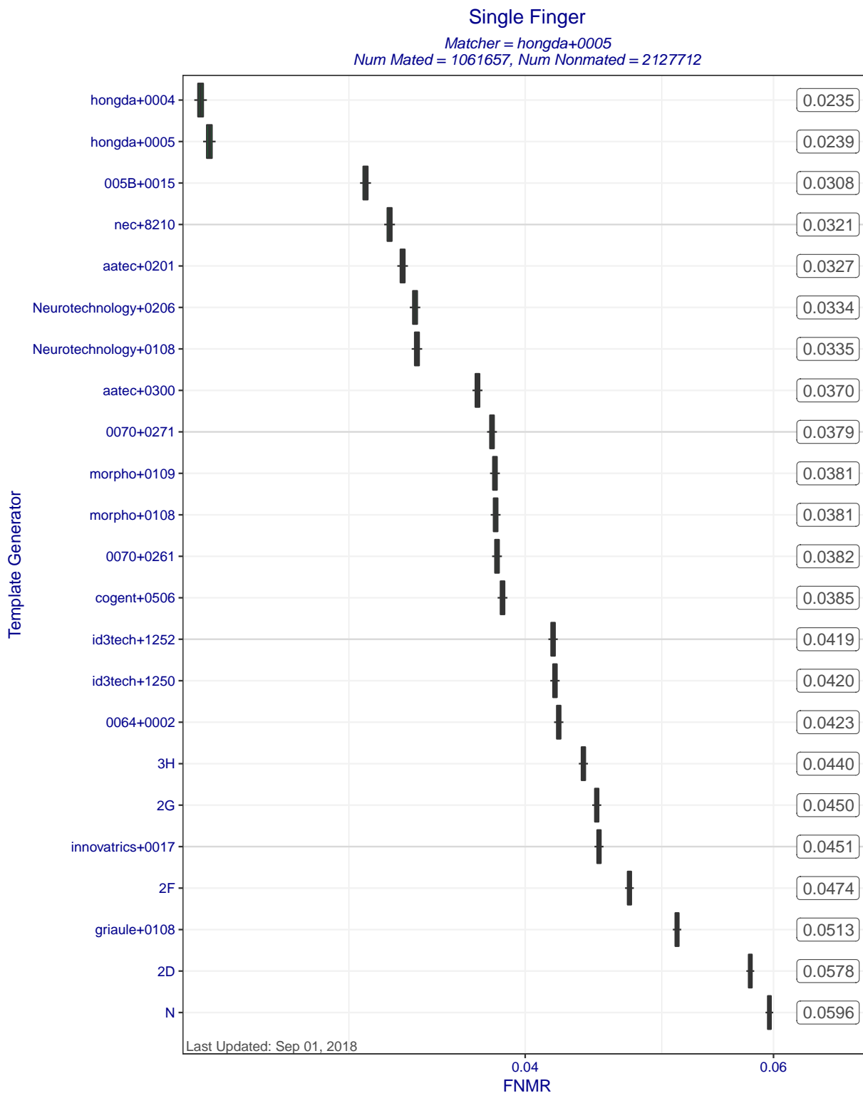
Figure 5: Single finger FNMRs at FMR = 0.0001 when matcher hongda+0005 compares templates created by different template generators. The ends of the whiskers show the minimum and maximum FNMRs. Each box represents uncertainty about the true FNMR. The box edges mark the 50% confidence intervals while the whiskers mark the 90% confidence intervals. The numbers on the right show the actual computed FNMRs.
