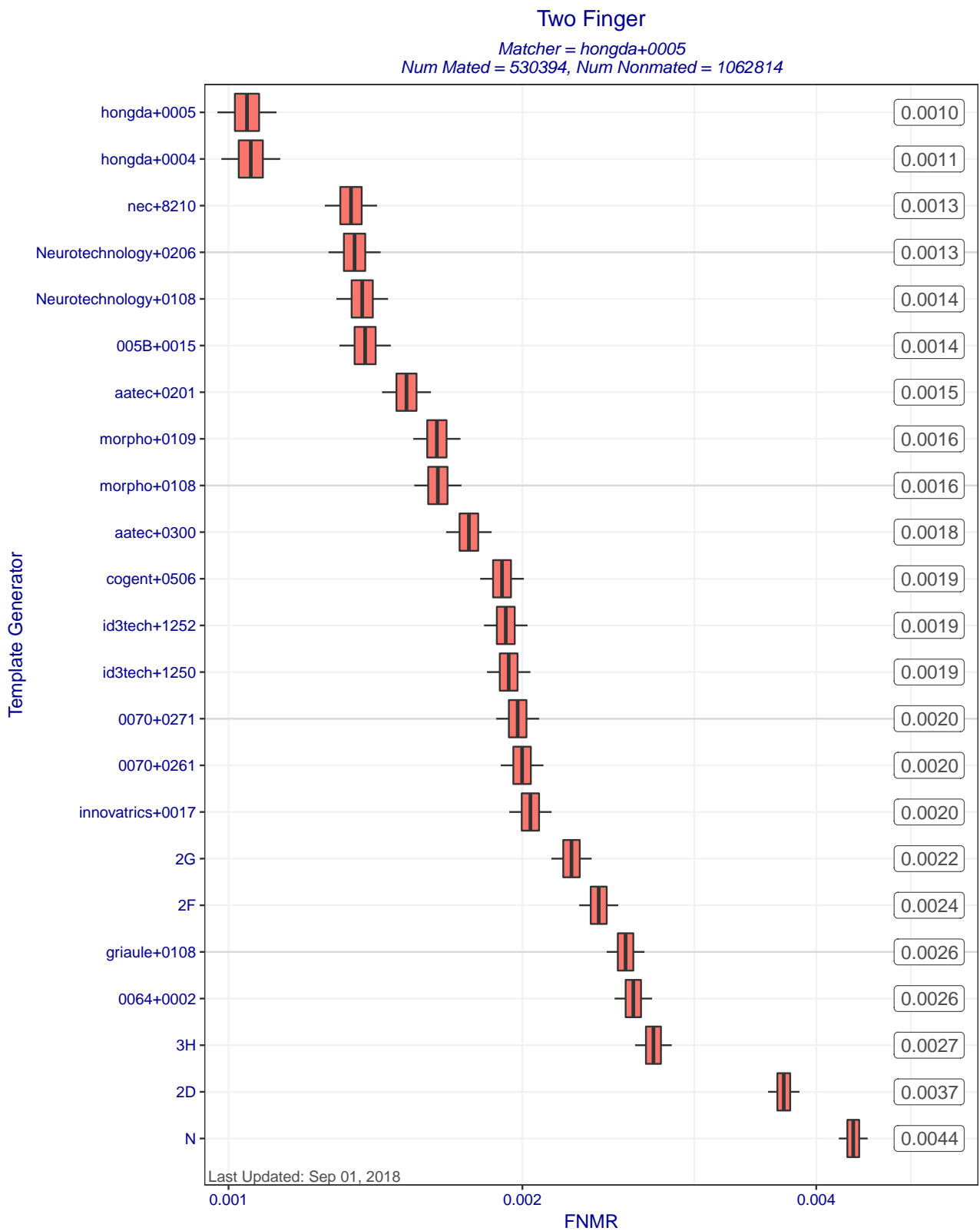
Figure 8: Two finger FNMR at FMR=0.01 when matcher hongda+0005 compares templates created by different template generators. Each box represents uncertainty about the true FNMR. The box edges mark the 50% confidence intervals while the whiskers mark the 90% confidence intervals. The numbers on the right show the actual computed FNMRs. Score-level fusion is achieved by averaging the scores for left and right index fingers.
