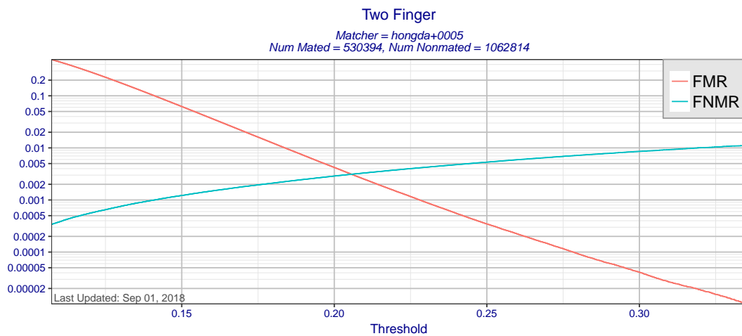
Figure 12: Two finger FMR and FNMR as a function of score threshold for matcher hongda+0005 using templates created by all MINEX III compliant template generators. Score-level fusion is achieved by averaging scores for the left and right index fingers.
