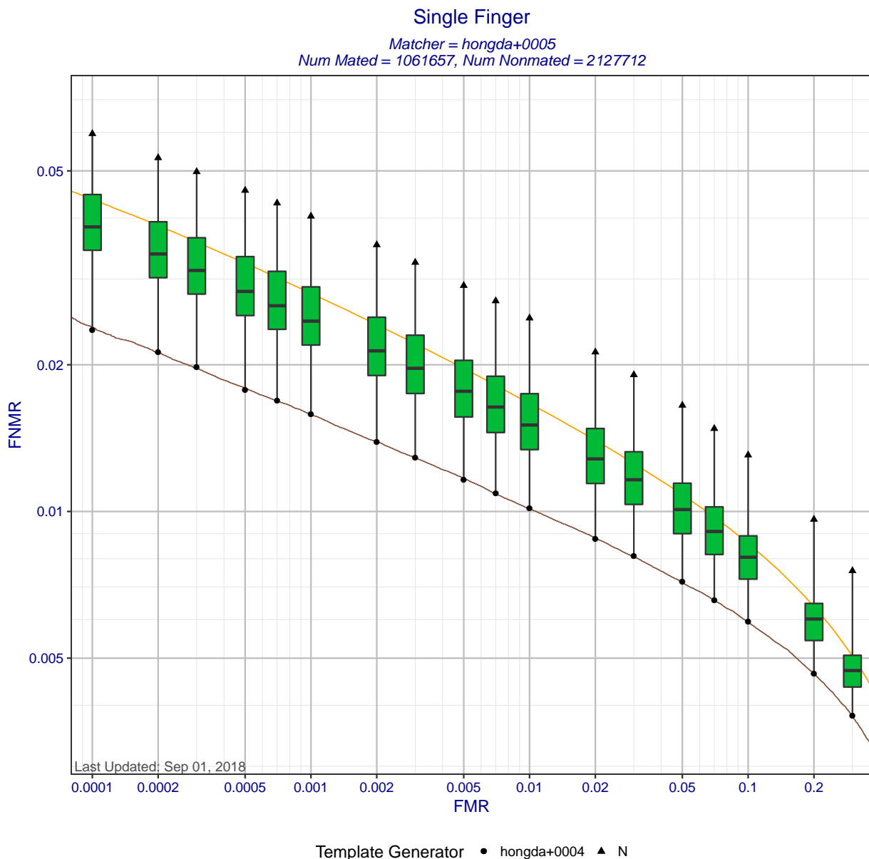
Figure 2: Single finger DET statistics for matcher hongda+0005. Each box shows the distribution of FNMRs at a fixed FMR across all MINEX III compliant template generators. The ends of the whiskers show the minimum and maximum FNMRs. The orange DET curve shows pooled performance against all template generators.
