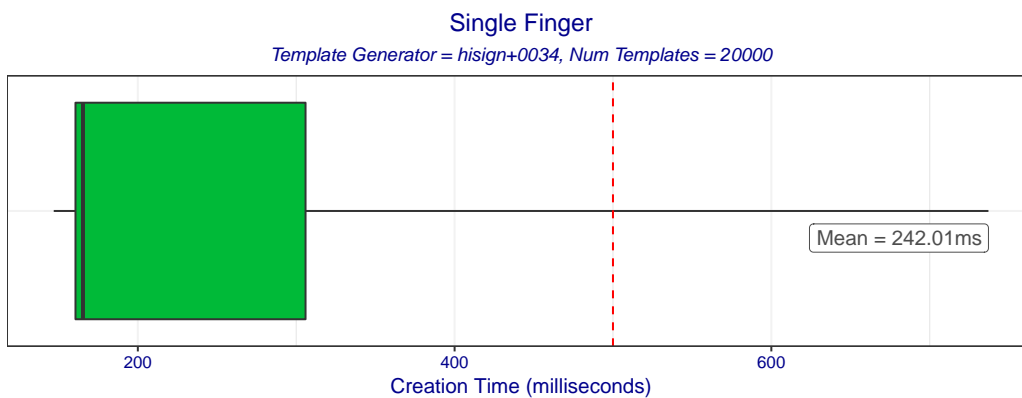
Figure 2: Boxplot of template creation times for template generator hisign+0034. The box edges mark the 10th and 90th percentiles while the whiskers mark the maximum and minimum creation times.
