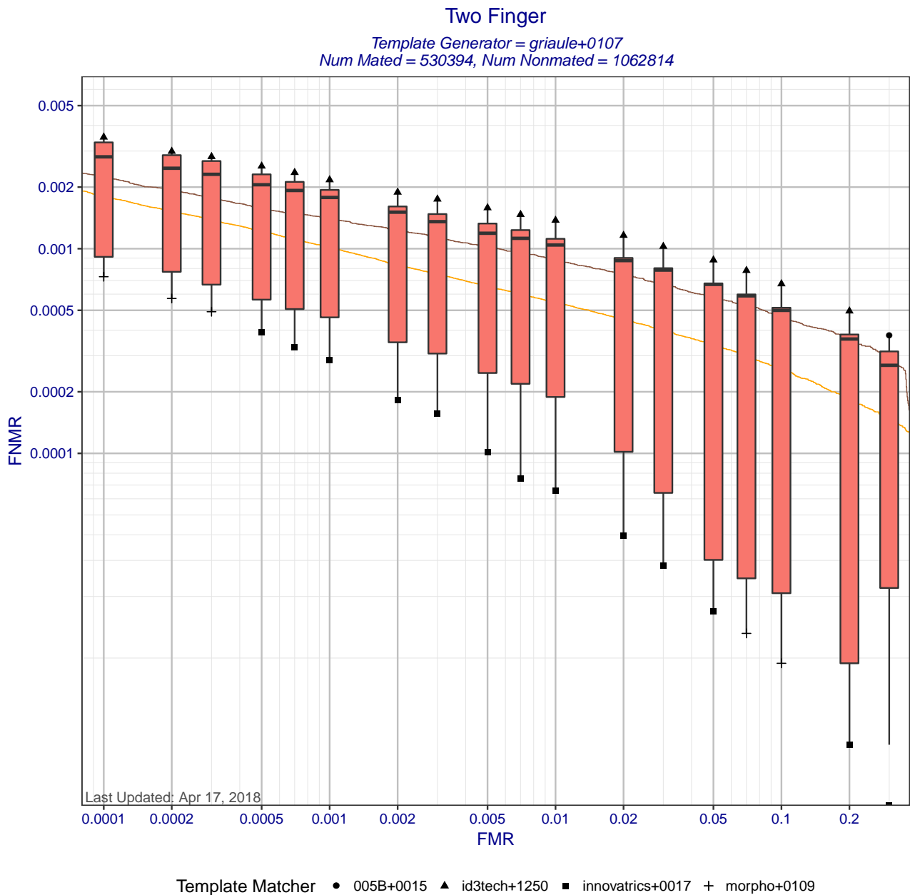
Figure 6: Two Finger DET statistics for template generator griaule+0107. Each box shows the distribution of FNMRs at a fixed FMR across different matchers. The whisker ends show the minimum and maximum FNMRs. The brown curve shows the DET curve when the matcher and template generators were submitted by the same participant. The orange DET curve shows pooled performance when all matchers use templates created by griaule+0107. Score-level fusion is achieved by averaging the scores for left and right index fingers.
