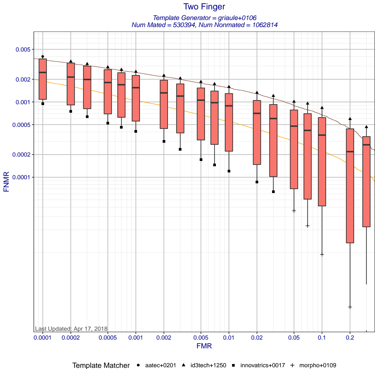
Figure 6: Two Finger DET statistics for template generator griaule+0106. Each box shows the distribution of FNMRs at a fixed FMR across different matchers. The whisker ends show the minimum and maximum FNMRs. The brown curve shows the DET curve when the matcher and template generators were submitted by the same participant. The orange DET curve shows pooled performance when all matchers use templates created by griaule+0106. Score-level fusion is achieved by averaging the scores for left and right index fingers.
