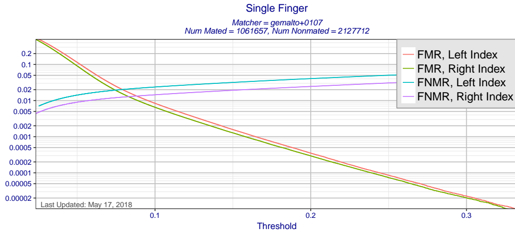
Figure 11: Single finger FMR and FNMR as a function of score threshold for matcher gemalto+0107 using templates created by all MINEX III compliant template generators. Separate curves are presented for left and right index fingers.
