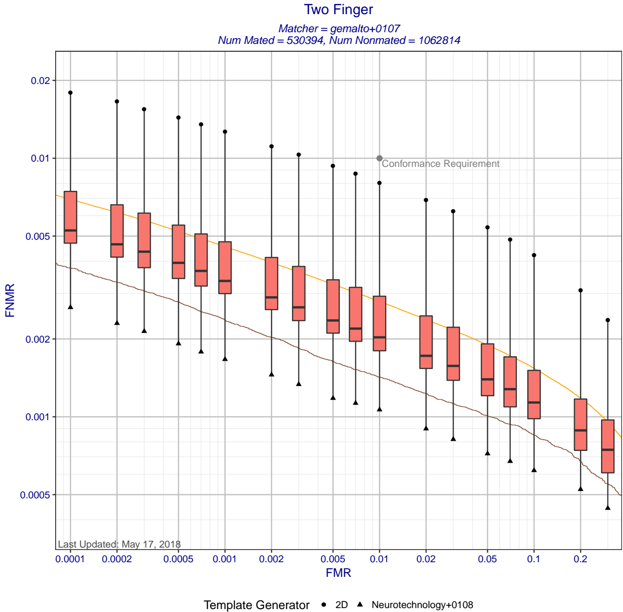
Figure 7: Two finger DET statistics for matcher gemalto+0107. Each box shows the distribution of FNMRs at a fixed FMR across all MINEX III compliant template generators. The whisker ends show the minimum and maximum FNMRs. The orange DET curve shows pooled performance against all template generators. Score-level fusion is achieved by averaging the scores for left and right index fingers.
