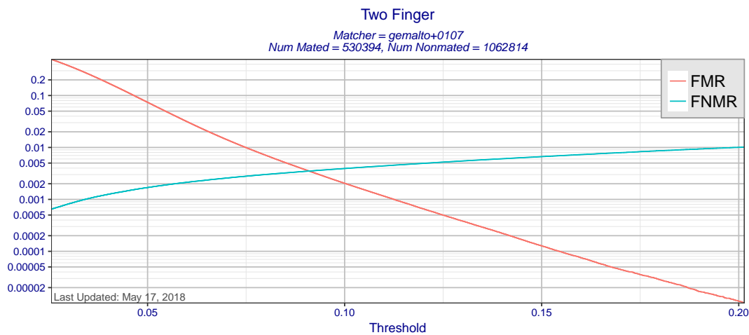
Figure 12: Two finger FMR and FNMR as a function of score threshold for matcher gemalto+0107 using templates created by all MINEX III compliant template generators. Score-level fusion is achieved by averaging scores for the left and right index fingers.
