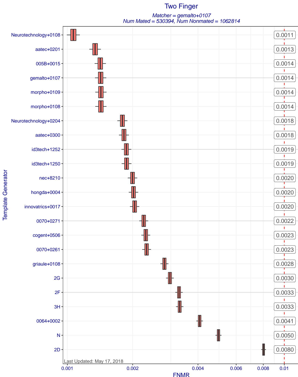
Figure 8: Two finger FNMR at FMR=0.01 when matcher gemalto+0107 compares templates created by different template generators. Each box represents uncertainty about the true FNMR. The box edges mark the 50% confidence intervals while the whiskers mark the 90% confidence intervals. The numbers on the right show the actual computed FNMRs. Score-level fusion is achieved by averaging the scores for left and right index fingers.
