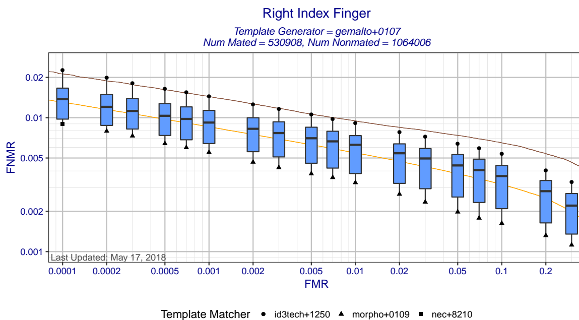
Figure 3: Right Index Finger DET statistics for template generator gemalto+0107. Each box shows the distribution of FNMRs at a fixed FMR across different matchers. The whisker ends show the minimum and maximum FNMRs. The brown curve shows the DET curve when the matcher and template generators were submitted by the same participant. The orange DET curve shows pooled performance when all matchers use templates created by gemalto+0107.
