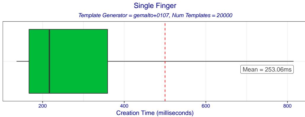
Figure 8: Boxplot of template creation times for template generator gemalto+0107. The box edges mark the 10th and 90th percentiles while the whiskers mark the maximum and minimum creation times.
