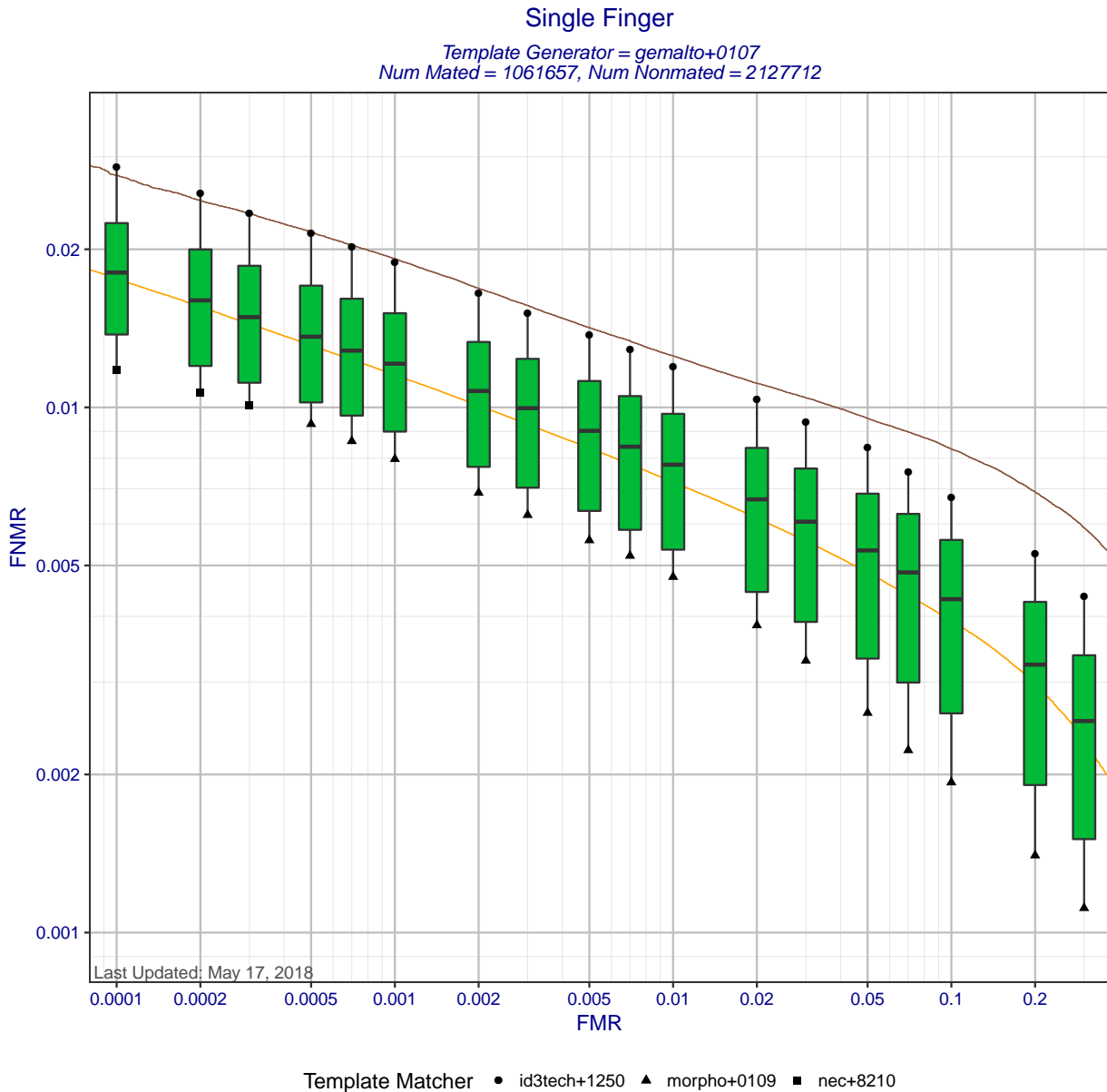
Figure 2: Single finger DET statistics for template generator gemalto+0107. Each box shows the distribution of FNMRs at a fixed FMR across different matchers. The whisker ends show the minimum and maximum FNMRs. The brown curve shows the DET curve when the matcher and template generators were submitted by the same participant. The orange DET curve shows pooled performance when all matchers compare templates created by gemalto+0107.
