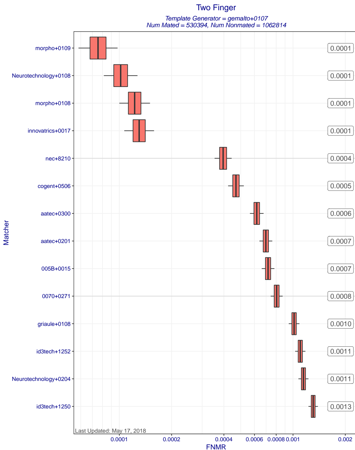
Figure 7: Two Finger FNMR at FMR=0.01 when different matchers compare templates created by template generator gemalto+0107. Each box represents uncertainty about the true FNMR. The box edges mark the 50% confidence intervals while the whiskers mark the 90% confidence intervals. The numbers on the right show the actual computed FNMRs. Score-level fusion is achieved by averaging the scores for left and right index fingers.
