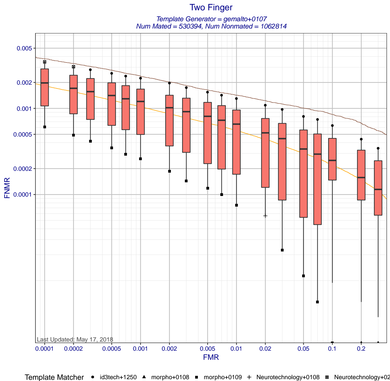
Figure 6: Two Finger DET statistics for template generator gemalto+0107. Each box shows the distribution of FNMRs at a fixed FMR across different matchers. The whisker ends show the minimum and maximum FNMRs. The brown curve shows the DET curve when the matcher and template generators were submitted by the same participant. The orange DET curve shows pooled performance when all matchers use templates created by gemalto+0107. Score-level fusion is achieved by averaging the scores for left and right index fingers.
