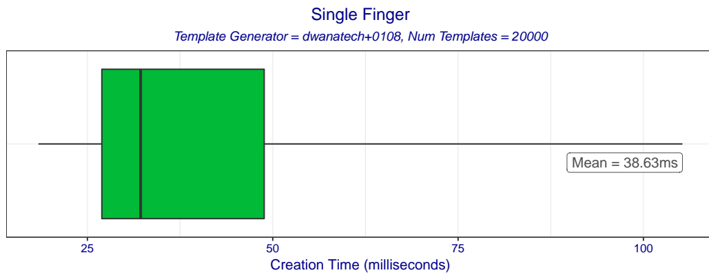
Figure 2: Boxplot of template creation times for template generator dwanatech+0108. The box edges mark the 10th and 90th percentiles while the whiskers mark the maximum and minimum creation times.
