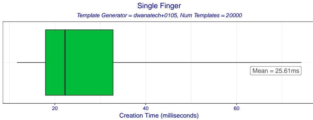
Figure 2: Boxplot of template creation times for template generator dwanatech+0105. The box edges mark the 10th and 90th percentiles while the whiskers mark the maximum and minimum creation times.
