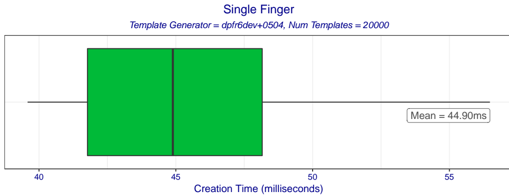
Figure 2: Boxplot of template creation times for template generator dpfr6dev+0504. The box edges mark the 10th and 90th percentiles while the whiskers mark the maximum and minimum creation times.
