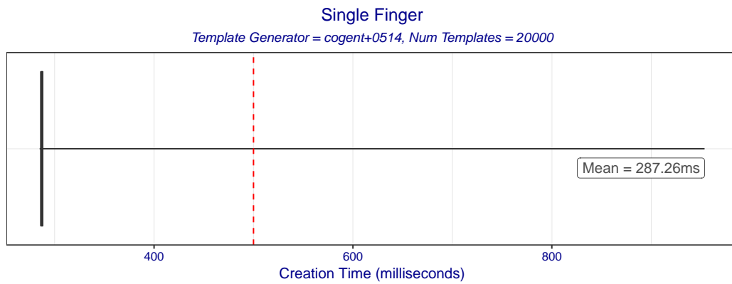
Figure 2: Boxplot of template creation times for template generator cogent+0514. The box edges mark the 10th and 90th percentiles while the whiskers mark the maximum and minimum creation times.
